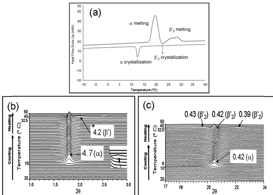
Fig. S1 showing the DSC thermogram and SR-XRD patterns obtained when POP was cooled at 2^\circ\text{C min}^{-1} and heated at 15^\circ\text{C min}^{-1} .
