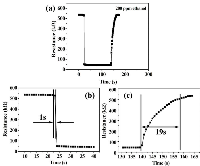
Fig. S2 Response transient of the sensor to 200 ppm ethanol.
