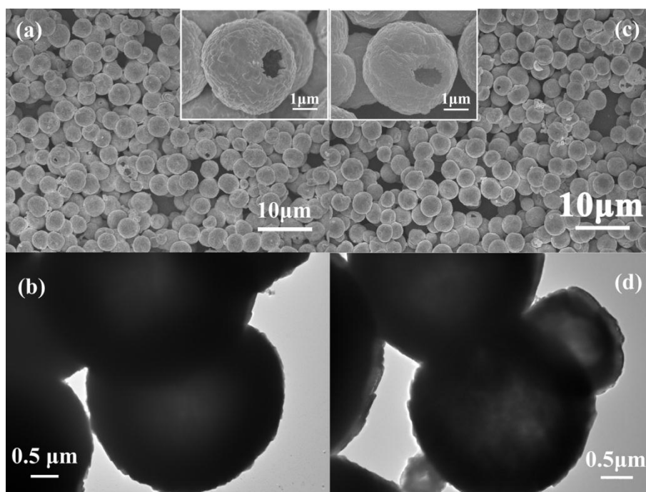
Fig. S1 Typical SEM and TEM images of uncalcined ZnO (a-b) and calcined ZnO (c-d) hollow microsphere.
