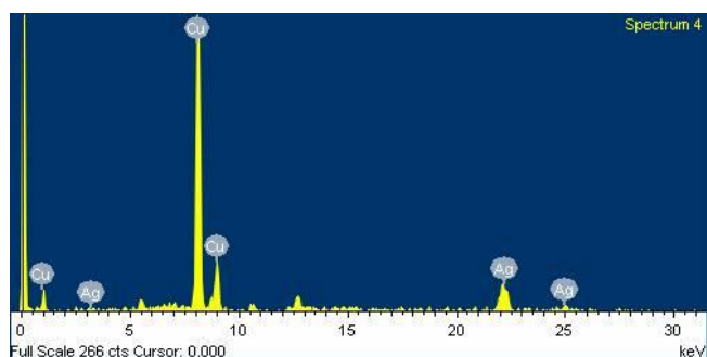
SI-2 EDS spectrum of the obtained product.
