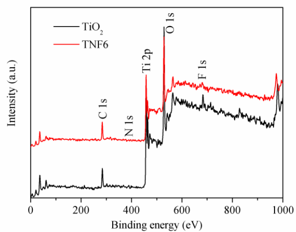
Fig. S1 Surface chemical composition of TiO 2 nanosheets and TNF6
