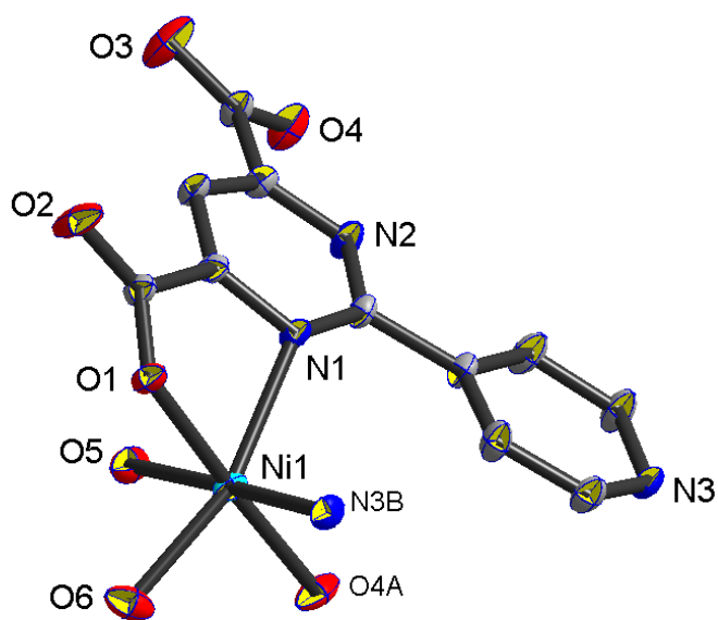
Figure S2. View of the coordination environment of the Ni1 center in 2 with a labeling scheme and 30% thermal ellipsoids.
