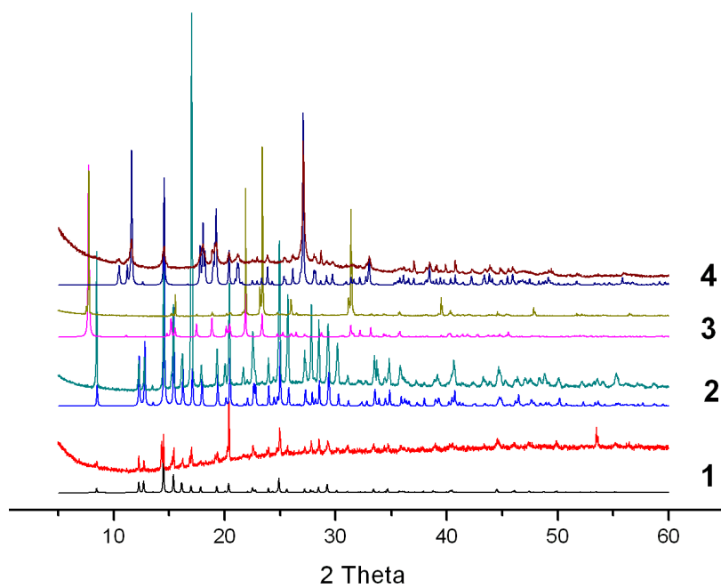
Figure S3. Comparison of the experimental and simulated PXRD patterns. In each group, the top is the experimental pattern and the bottom is the simulated one.
