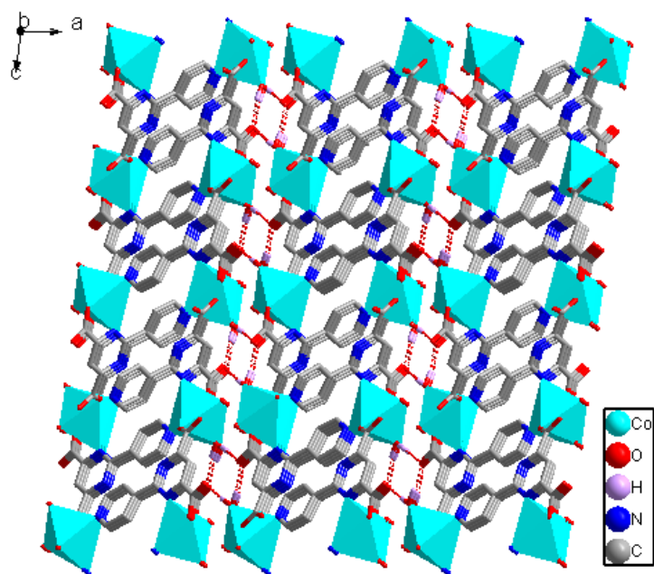
Figure S1. View of a 3D net in 1 looking along the b axis.
