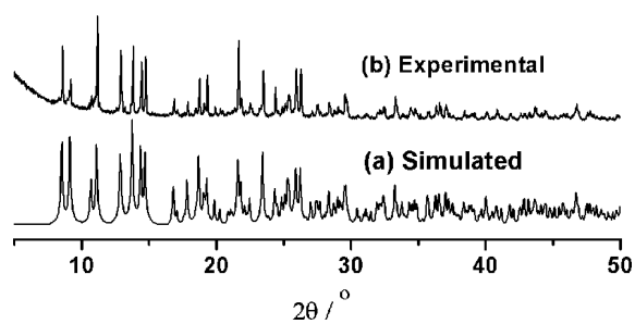
Figure S4 The experimental and simulated PXR D patterns for complex 4.
