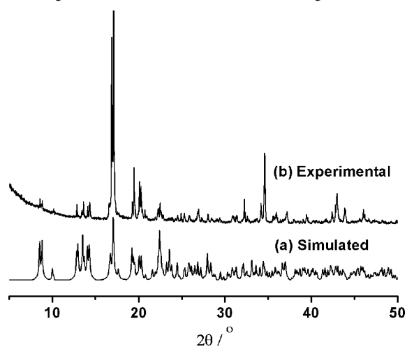
Figure S3 The experimental and simulated PXR D patterns for complex 3.
