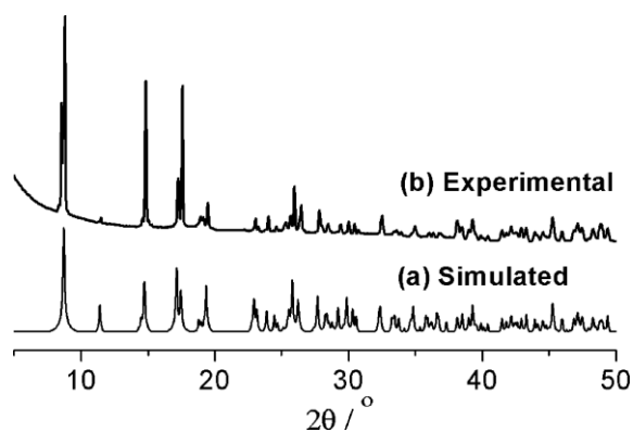
Figure S1 The experimental and simulated PXRD patterns for complex 1.
