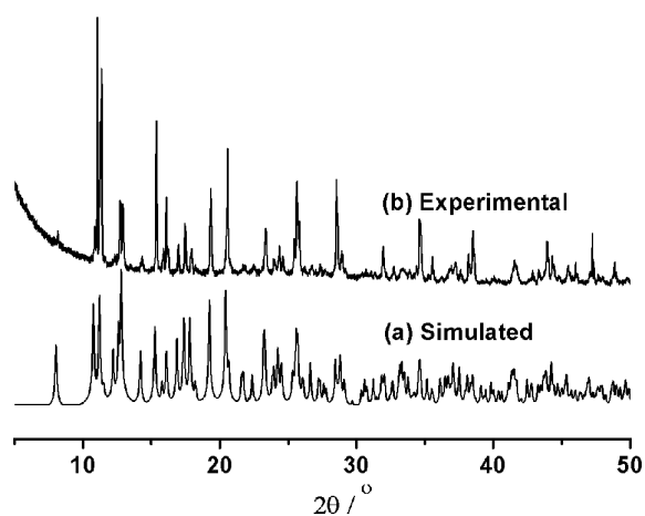
Figure S2 The experimental and simulated PXR D patterns for complex 2.
