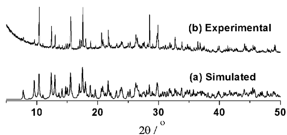
Figure S5 The experimental and simulated PXR D patterns for complex 5.
