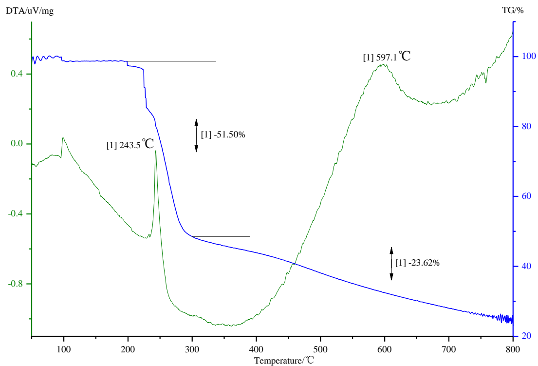
The TGA and DSC curves of 5
