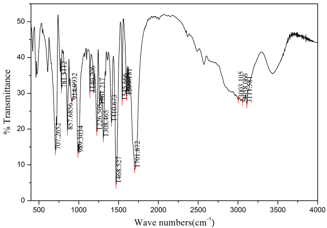
The IR curve of 6
