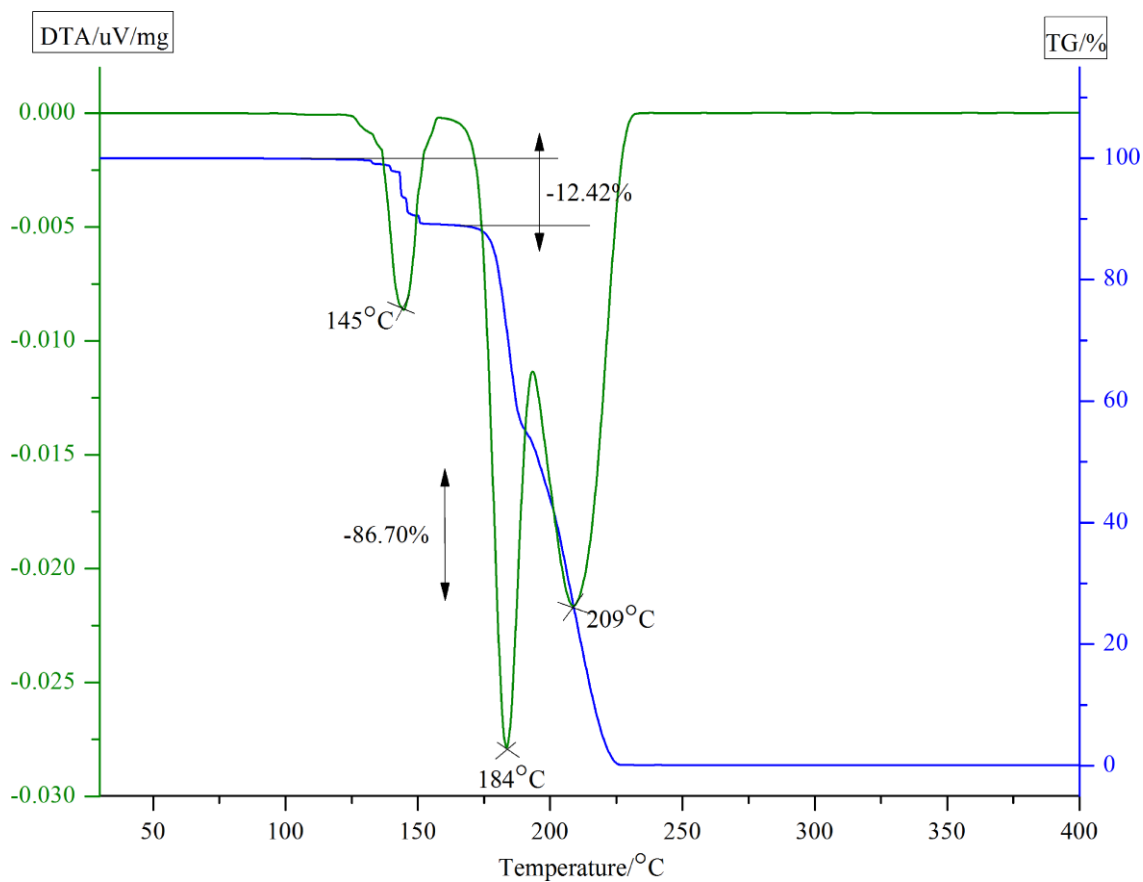
The TGA and DSC curves of 2
