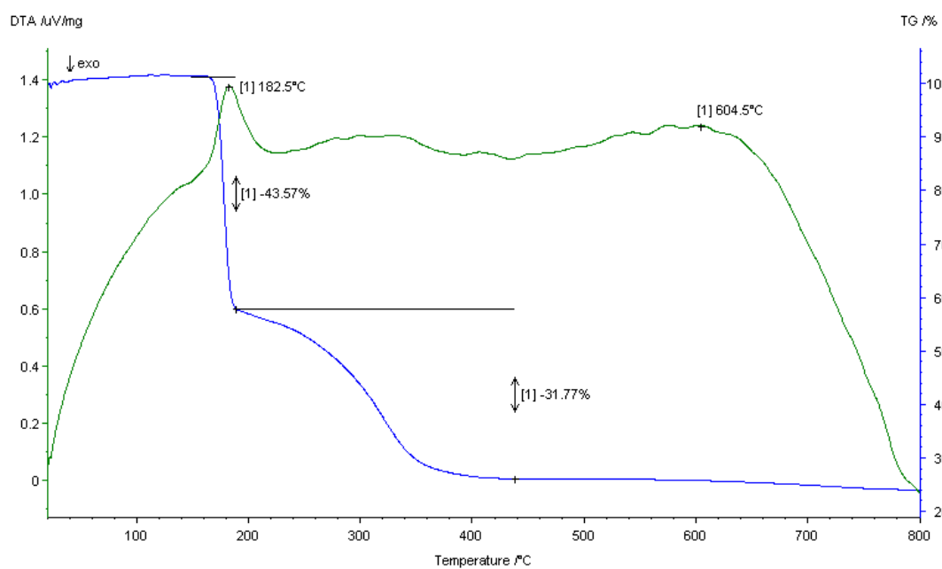
The TGA and DSC curves of 6
