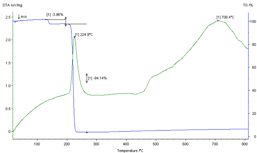
The TGA and DSC curves of 3
