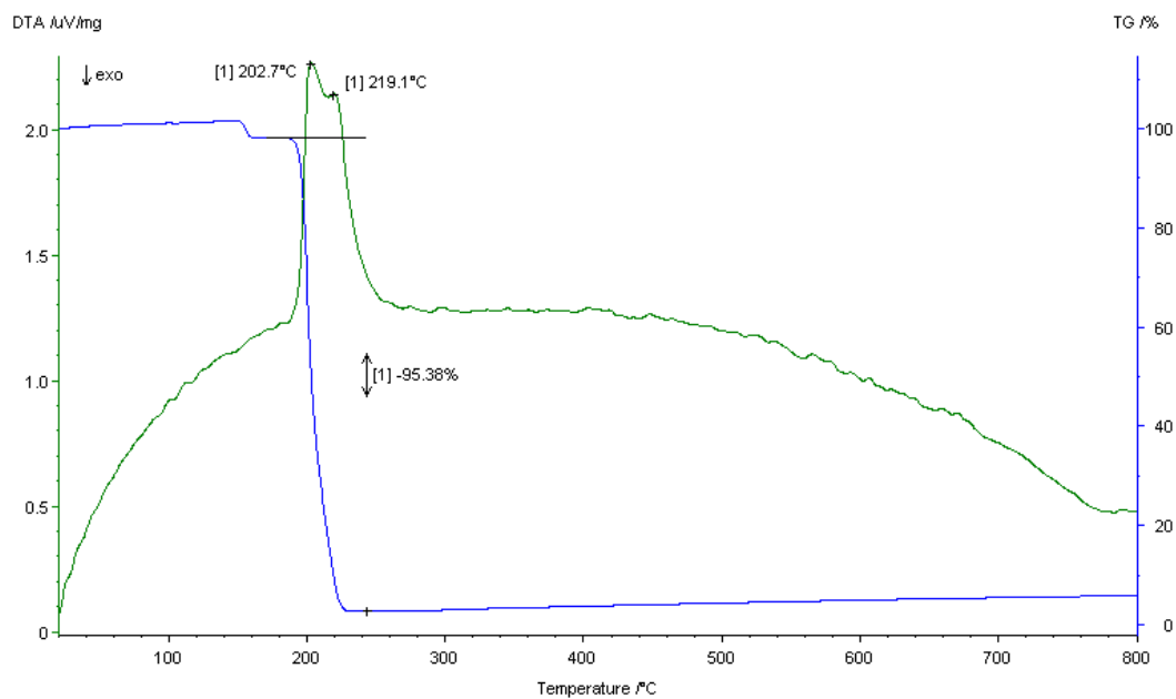
The TGA and DSC curves of 1
