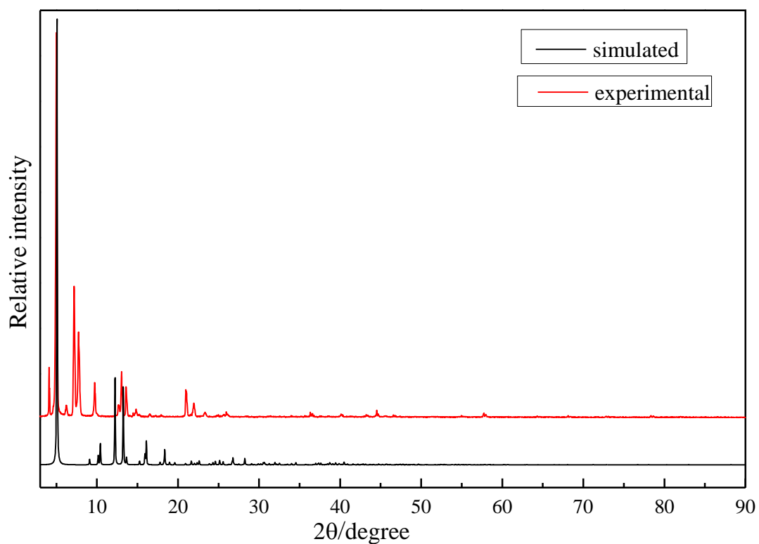
The XRD curve of 8
