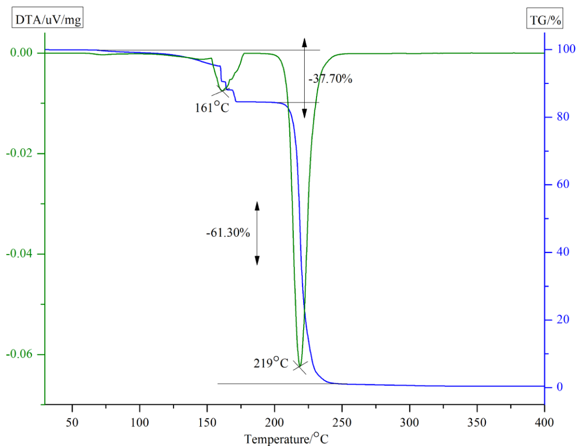
The TGA and DSC curves of 4
