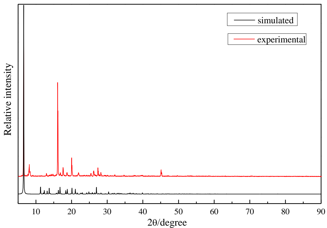
The XRD curve of 6
