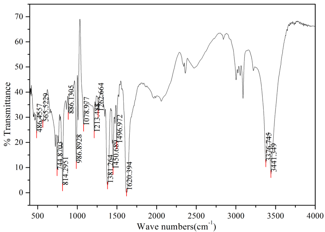
The IR curve of 4
