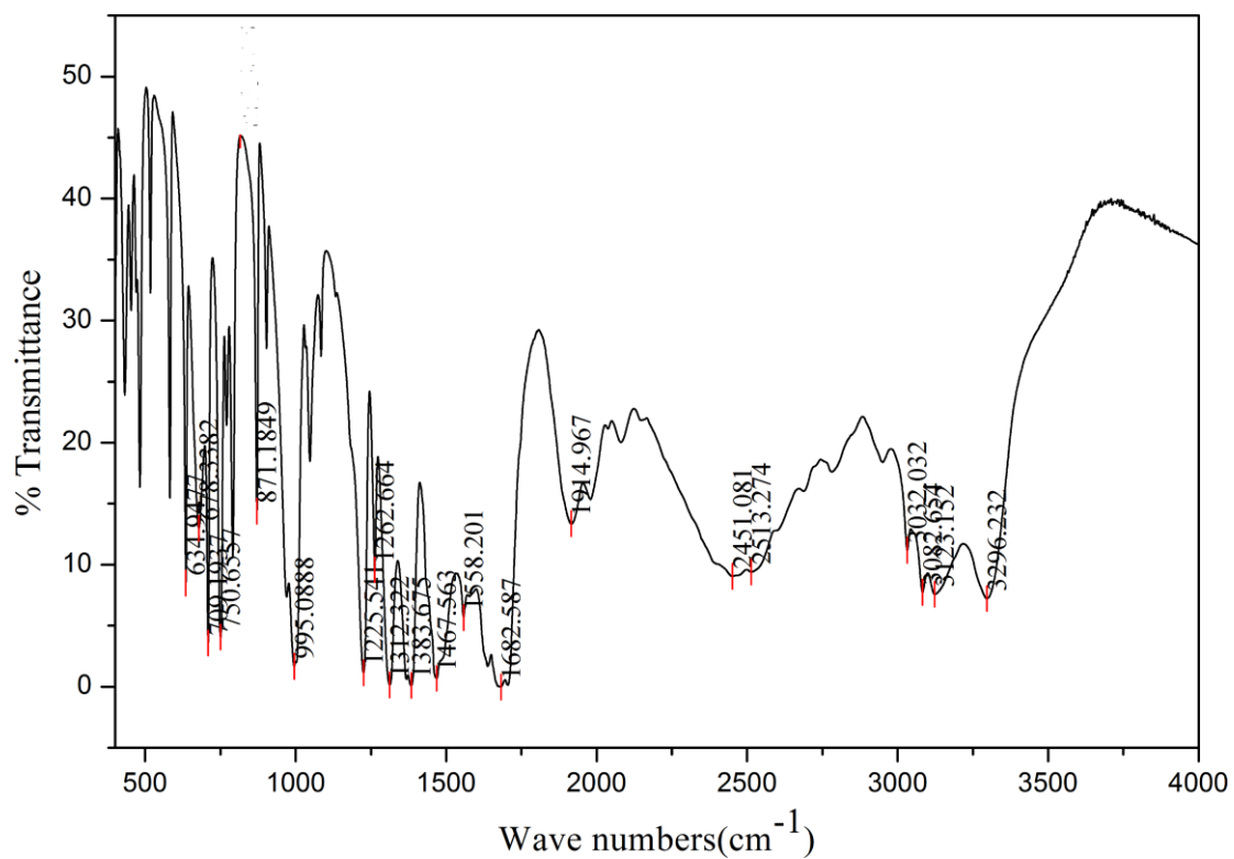
The IR curve of 3
