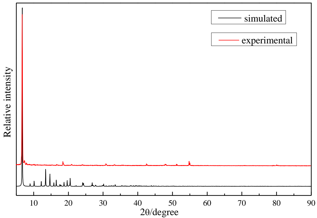
The XRD curve of 5
