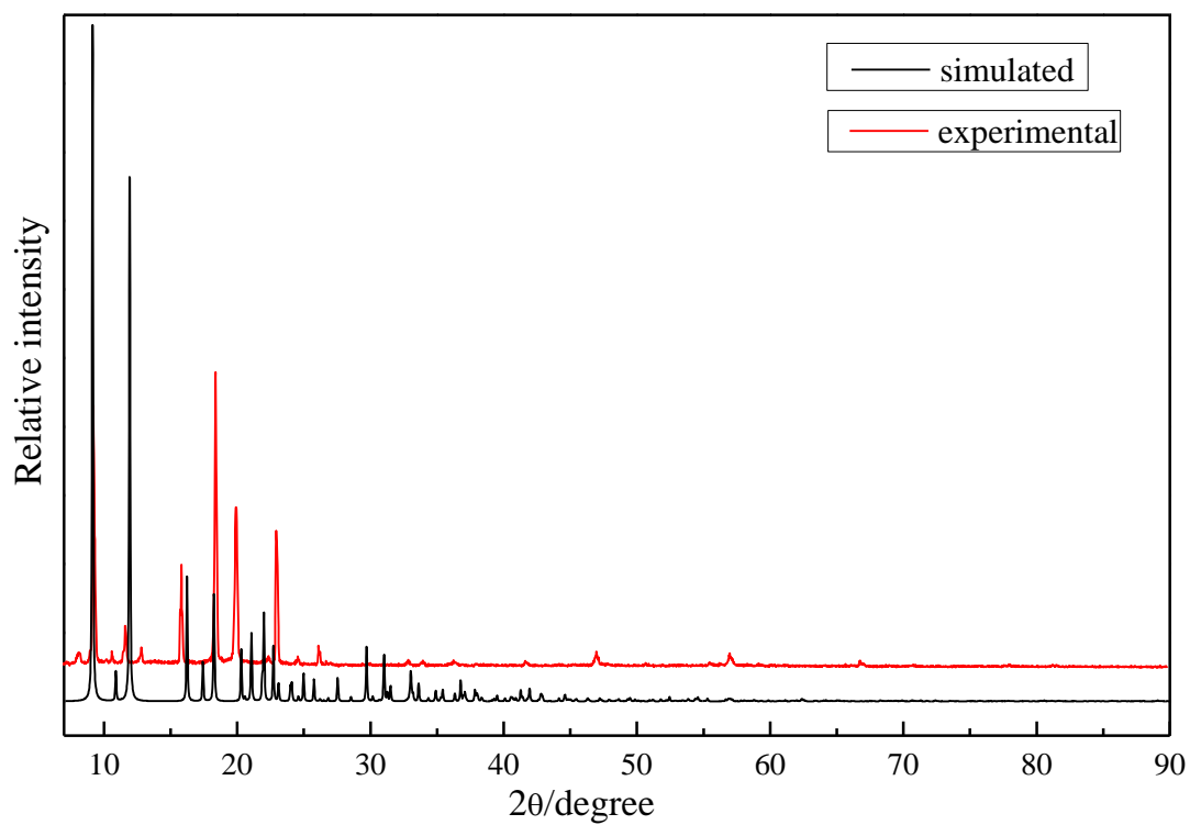
The XRD curve of 1
