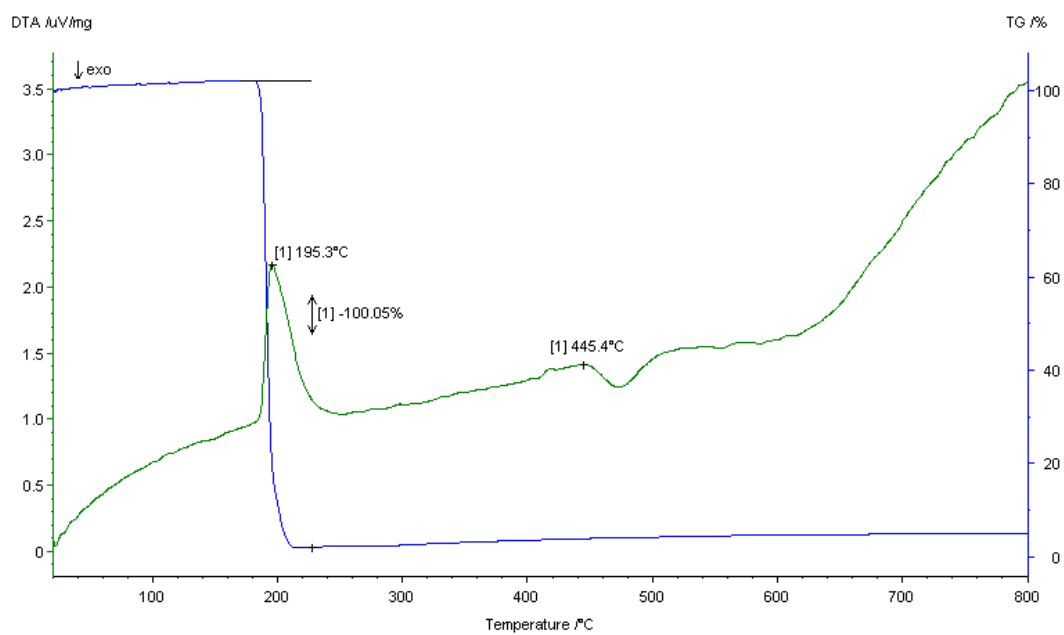
The TGA and DSC curves of 8
