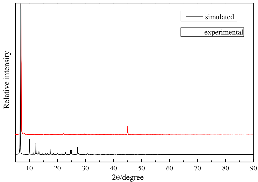
The XRD curve of 7
