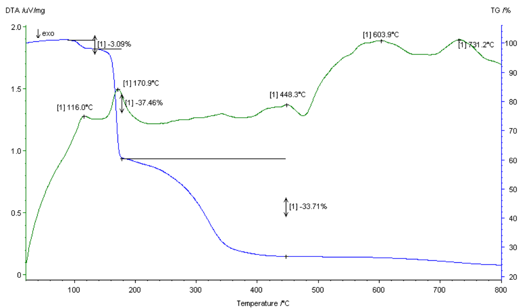
The TGA and DSC curves of 7
