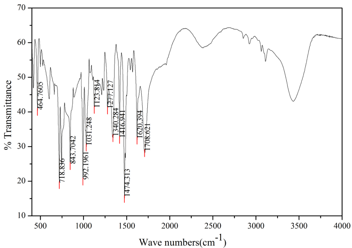
The IR curve of 5
