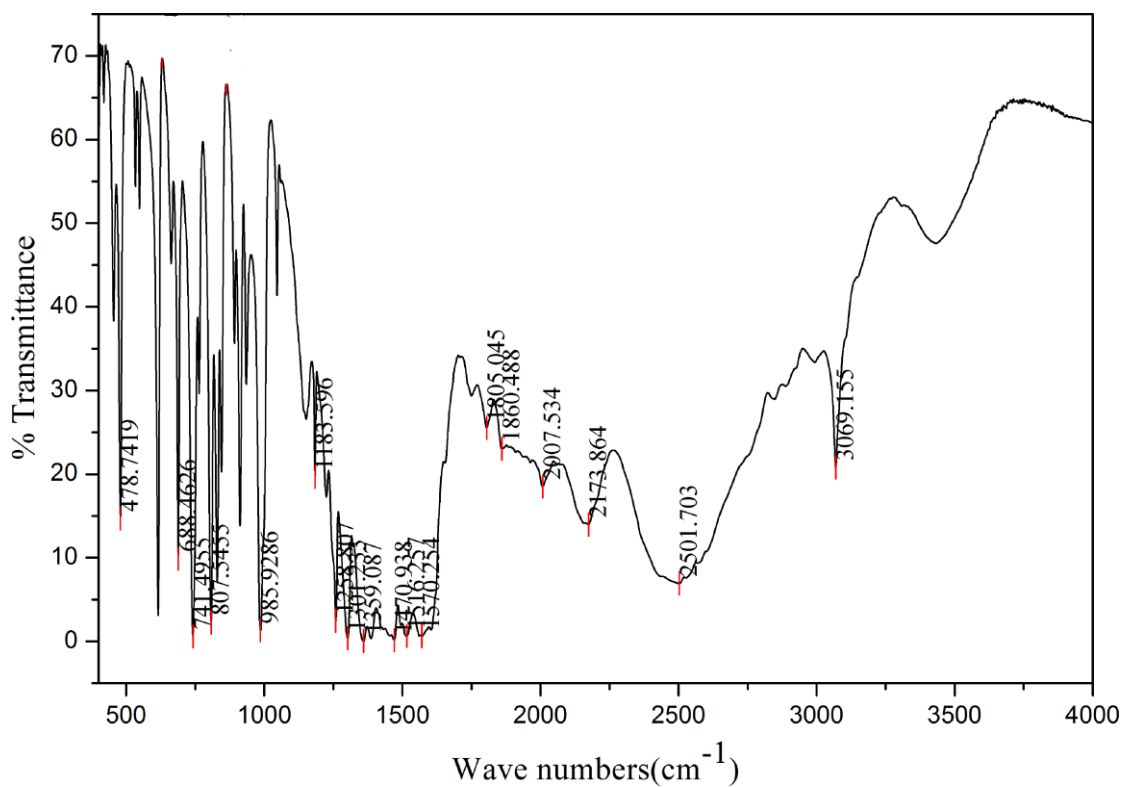
The IR curve of 1
