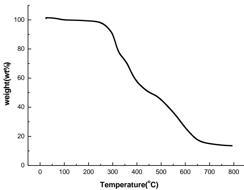
Figure S7 TGA curve of 7 .
