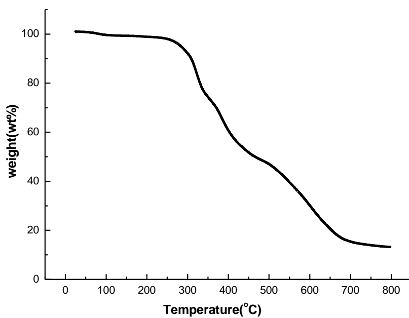
Figure S8 TGA curve of 8 .
