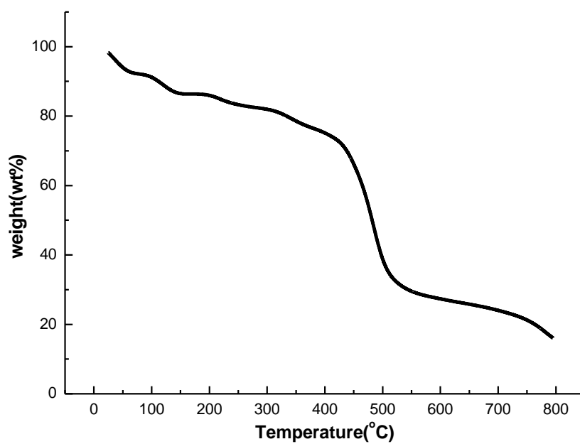
Figure S5 TGA curve of 5 .
