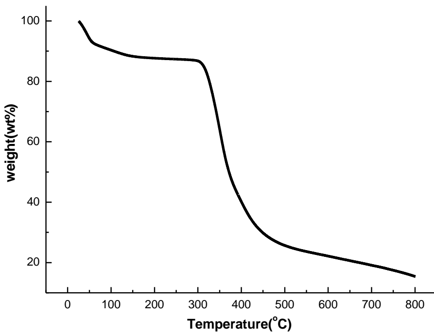
Figure S2 TGA curve of 2.
