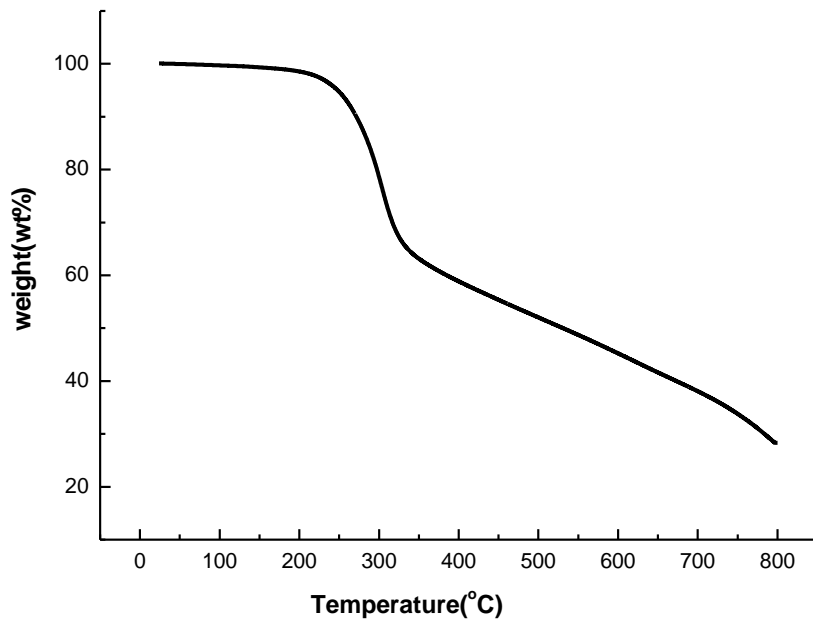
Figure S4 TGA curve of 4 .
