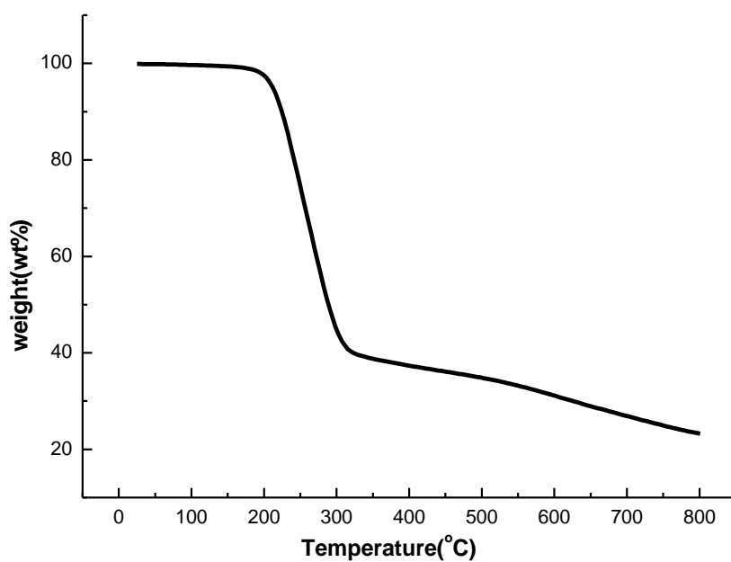
Figure S3 TGA curve of 3 .
