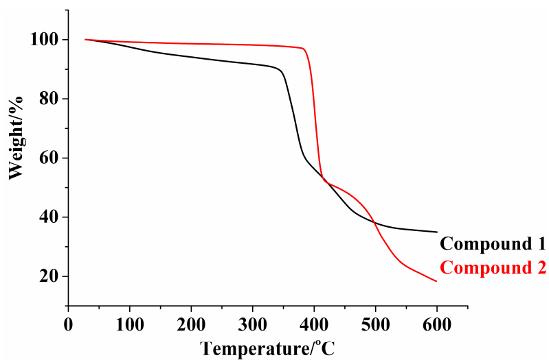
Fig. S3 TGA curves of compounds 1 and 2
