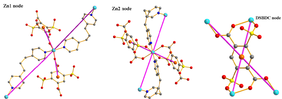
Fig. S1 Schematic view of the three types of 4-connected nodes in 1
