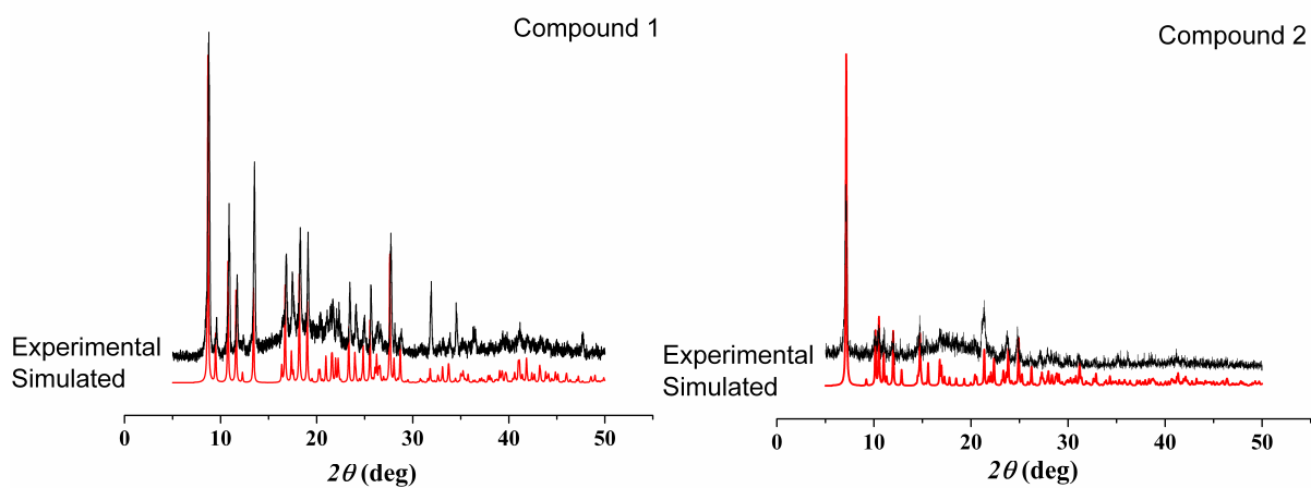
Fig. S4. Powder X-ray diffraction patterns of compounds 1 and 2
