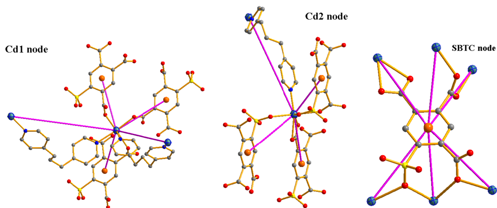
Fig. S2 Schematic view of the (4, 5, 6)-connected nodes in 2
