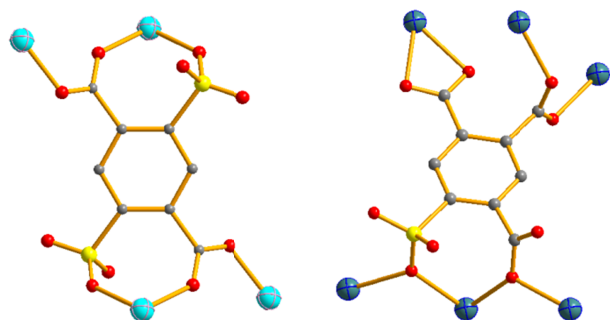
Scheme S1 The observed coordination modes of the DSBDC 4- and SBTC 4- ligands in compounds 1 and 2
