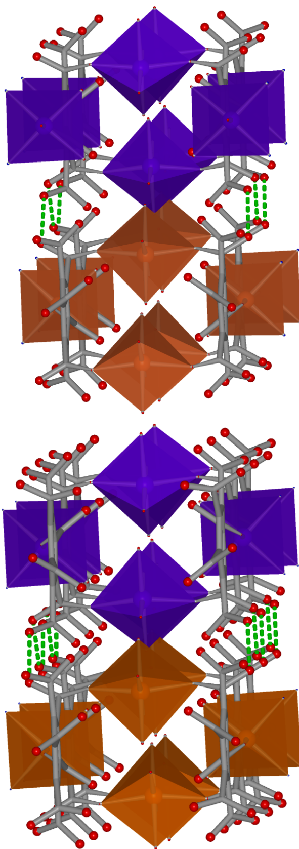
Figure S2. Hydrogen bonds between the 1D-SBUs in compounds 2 (top) and 3 (bottom).
