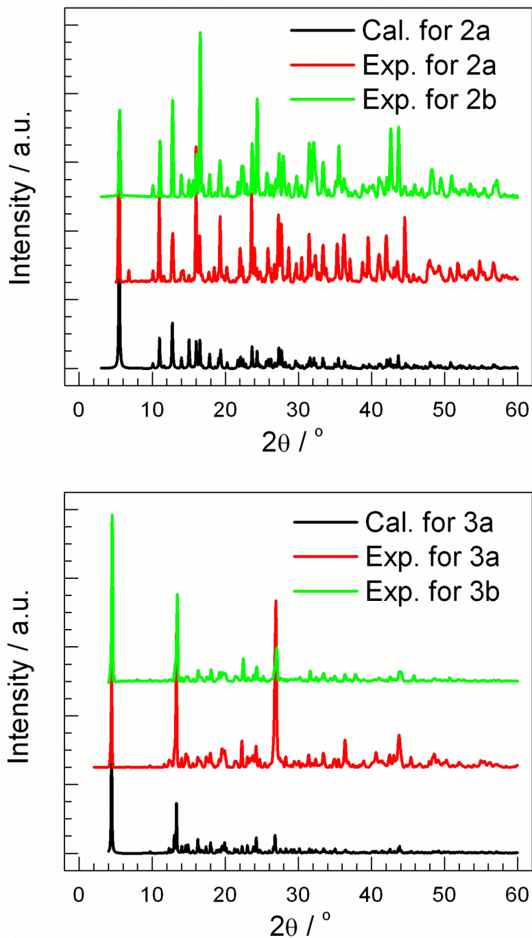
Figure S1. Calculated and experimental PXRD patterns for compounds 2a , 2b , 3a , and 3b
