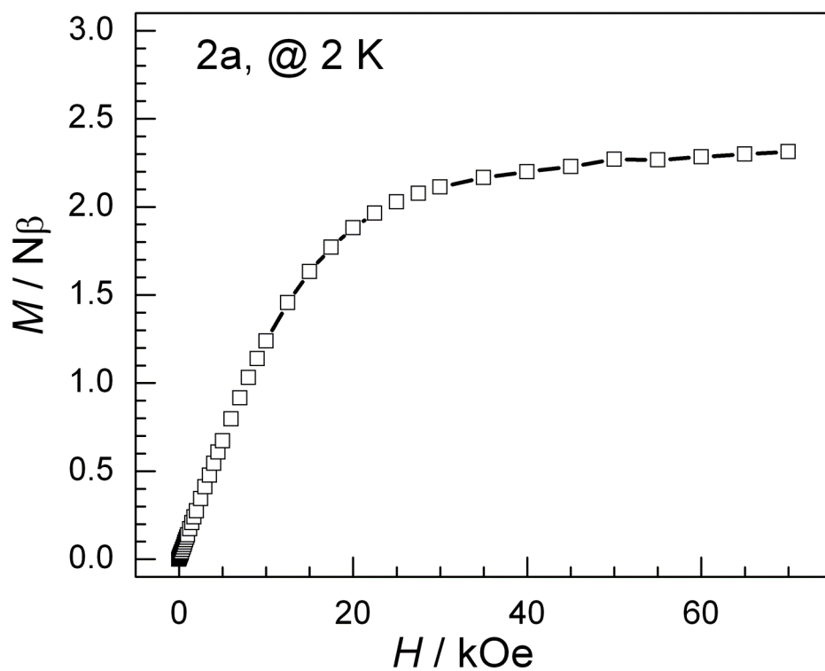
Figure S3. Magnetization vs. H at 2 K for 2a .
