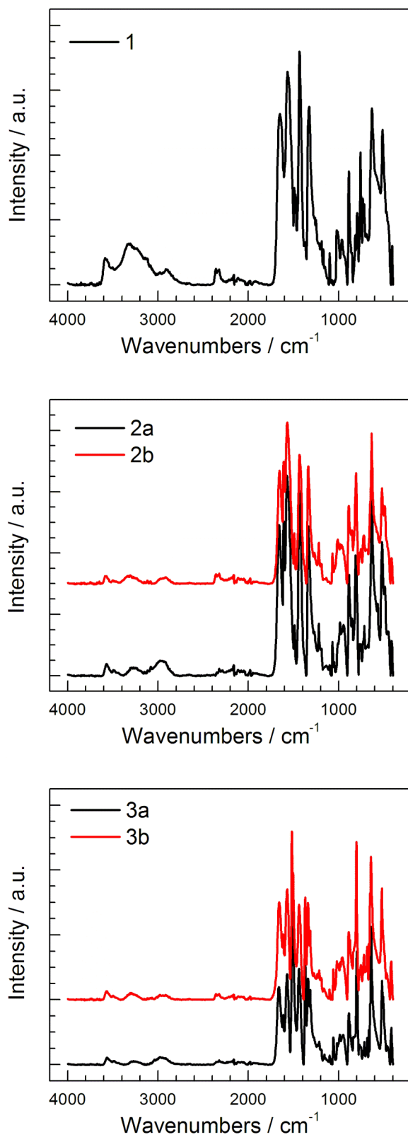
Figure S4. The IR spectra of the five compounds
