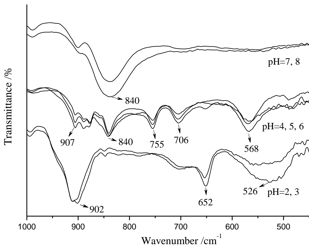
Figure S1. FI-IR spectra of the products synthesized at the condition of different pH values (2-8).
