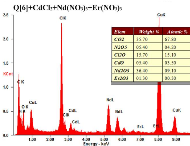
SI-1 The EDS spectra of precipitation in the Ln light /Ln heavy -Q[6]-[CdCl 4 ] 2- systems.
