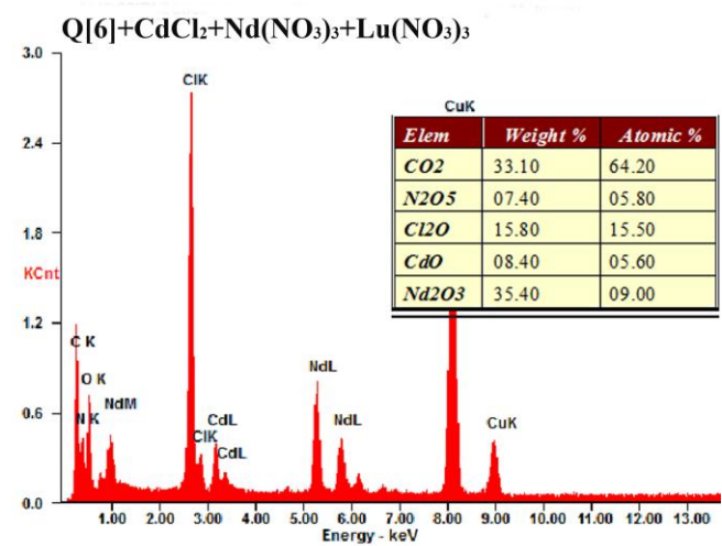
SI-1 The EDS spectra of precipitation in the Ln light /Ln heavy -Q[6]-[CdCl 4 ] 2- systems.
