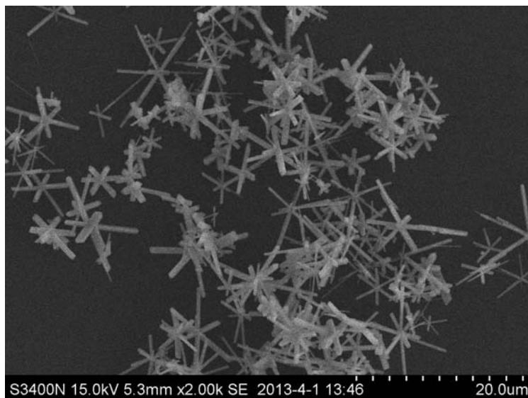
Figure S3 SEM image of MnOOH synthesized under a condition: 1 mmol MnSO 4 + 1.75 mmol KClO 3 + 0.1 mL AcOH; 15 mL distilled water; 12 h, 160 °C;
