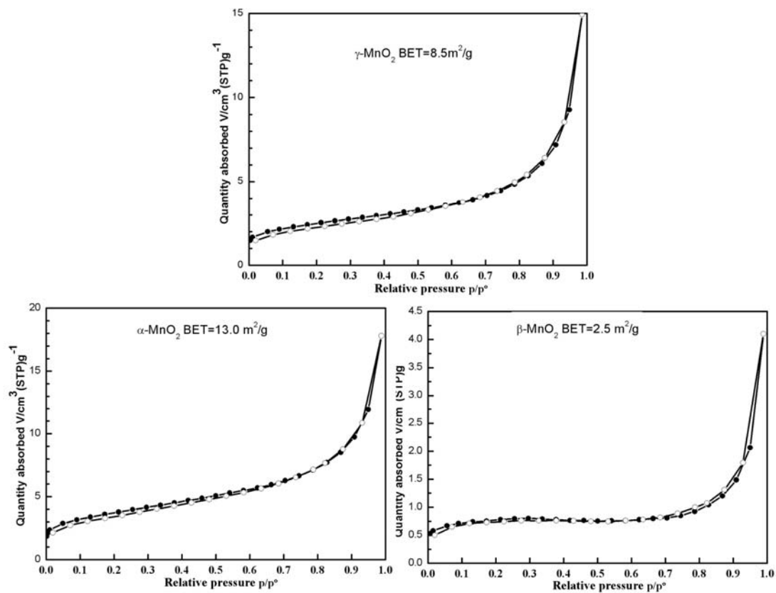
Figure S1 N 2 adsorption–desorption isotherms of manganese oxide
