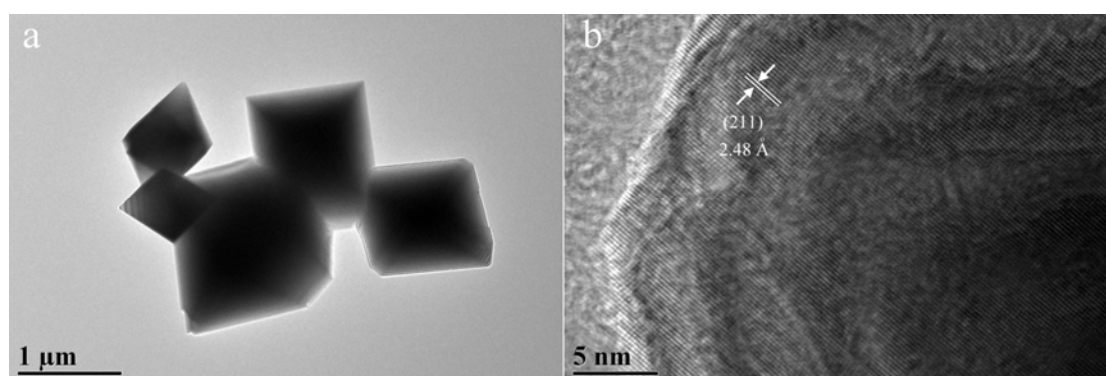
Figure S2 TEM and HRTEM images of \text{Mn}_3\text{O}_4
