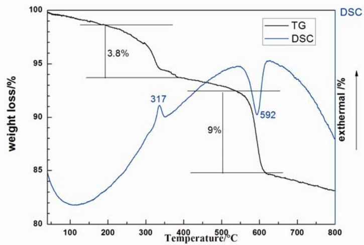
Figure S4 TG-DSC curves of MnOOH
