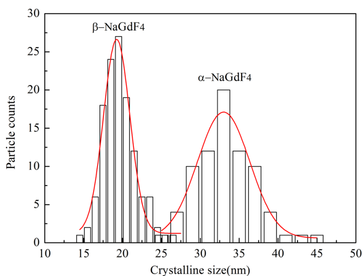
Fig.S1 Crystallite size distribution of \alpha -NaGdF 4 and \beta -NaGdF 4 nanocrystals in the glass ceramics
