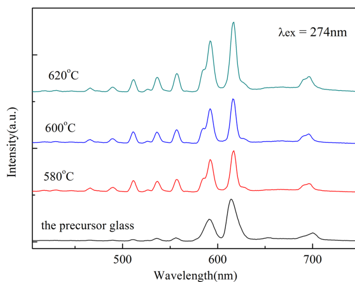
Fig.S3 Emission spectra of Eu 3+ ions in the precursor glass and glass ceramics ( x = 10 )
