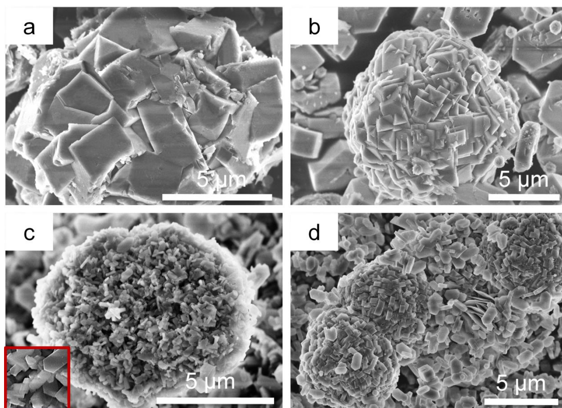
Fig. S1. The aggregation forms of ZSM-5 zeolites from various seed-assisted, template-free syntheses: (a) m-ZSM-5, (b) m-ZSM-11, (c) h-ZSM-5, (d) h-ZSM-11.
