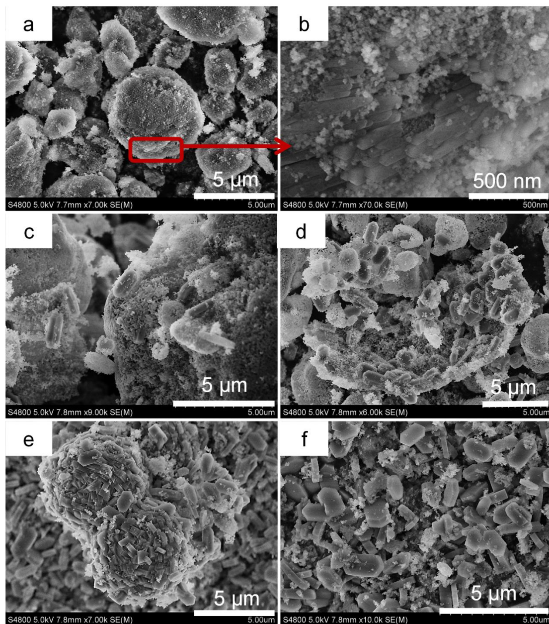
Fig. S2. The SEM images of samples obtained from various crystallization stages in the hierarchical ZSM-11-seeded synthesis system. (a-b) 170 °C for 0 h, (c-d) 170 °C for 8 h with RC of 39.18 %, (e-f) 170 °C for 10 h with RC of 77.47 %.
