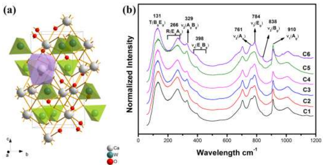
Fig. S1. (a) Unit cells of the standard \text{CaWO}_4 crystal. (b) FT-Raman spectrum of C1-C6 with different morphologies obtained by hydrothermal synthesis.
