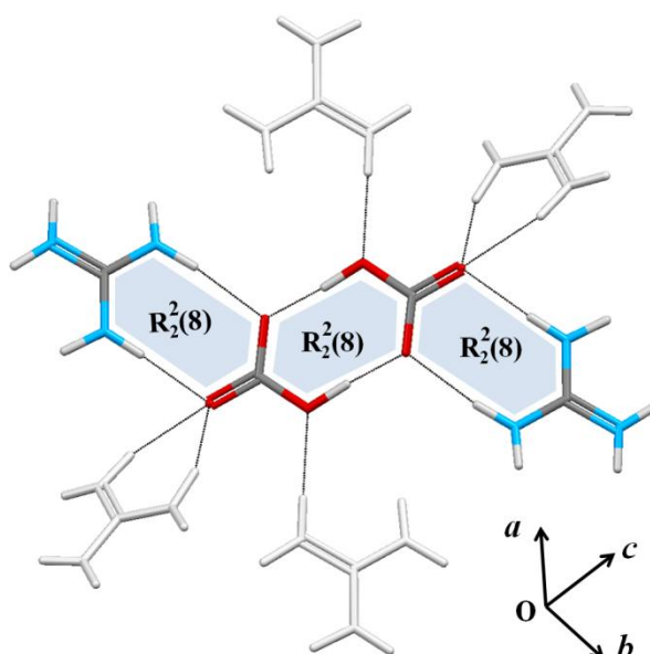
Fig. S2: Hydrogen-bonding network in guanidinium-bicarbonate (Refcode; DUMPUW). Partially related to the GIT structure.
