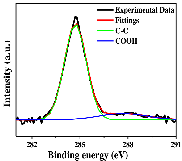
Fig. S2: XPS spectra of C 1S peak of the sample 48A after photocatalytic reaction.
