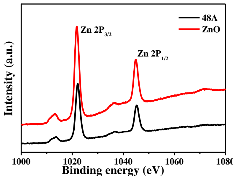
Fig. S1: XPS spectra of Zn 2P peak of the samples
