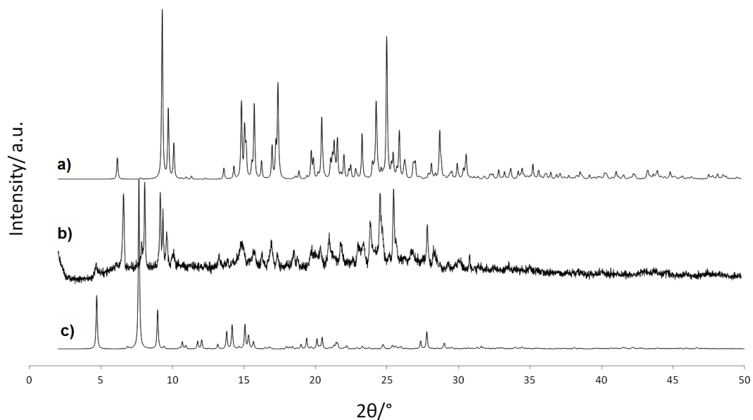
Fig. S1. a) The PXR pattern of 2 simulated from single crystal data, b) the experimental PXR for 2 and c) the PXR pattern of 3 simulated from single crystal data.
