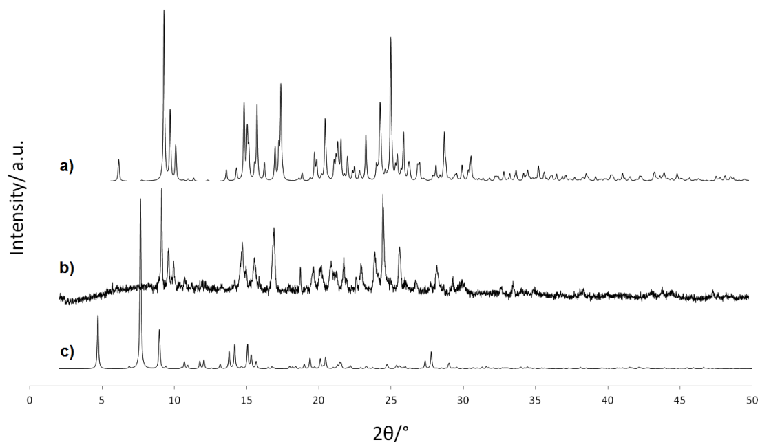
Fig. S1. a) The PXR pattern of 2 simulated from single crystal data, b) the experimental PXR for 2 and c) the PXR pattern of 3 simulated from single crystal data.
