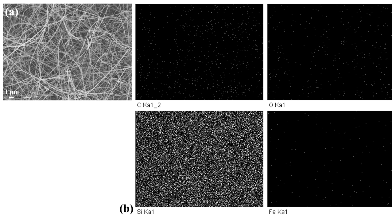
Fig. S1. (a) FESEM image and (b) mapping EDS results of the as-formed nanowires.
