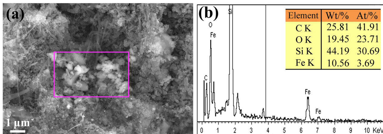
Fig. S2. (a) FESEM image and (b) EDS pattern of the cross-section areas on the Si substrate.
