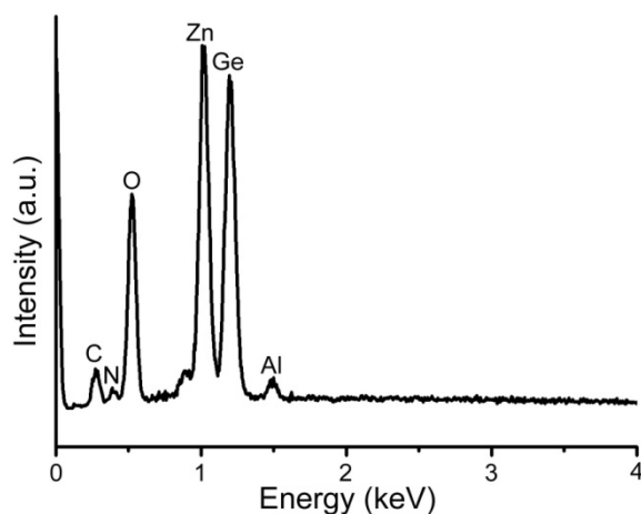
Figure S3, Typical EDS spectra taken from a single hybrid ZGO-DETA nanowire.
