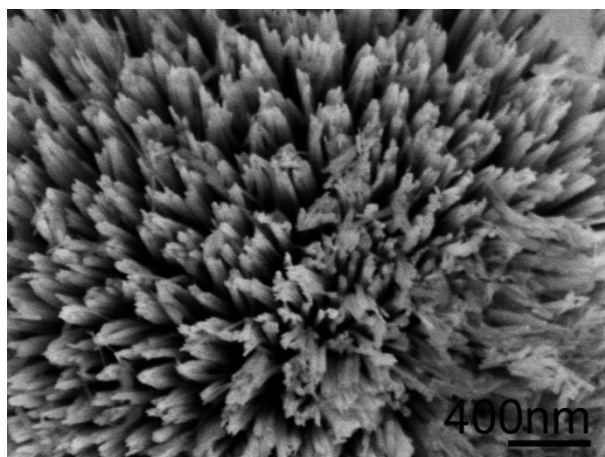
Figure S1. High-magnification SEM image of the ZGO-DETA hybrid.
