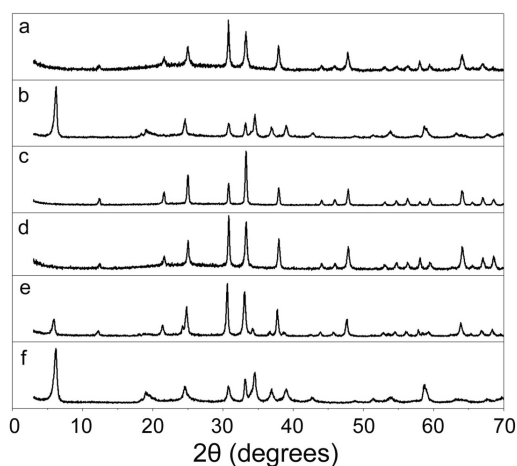
Figure S4. The X-ray diffraction (XRD) pattern of products synthesized under different synthetic conditions listed on Table 1.
