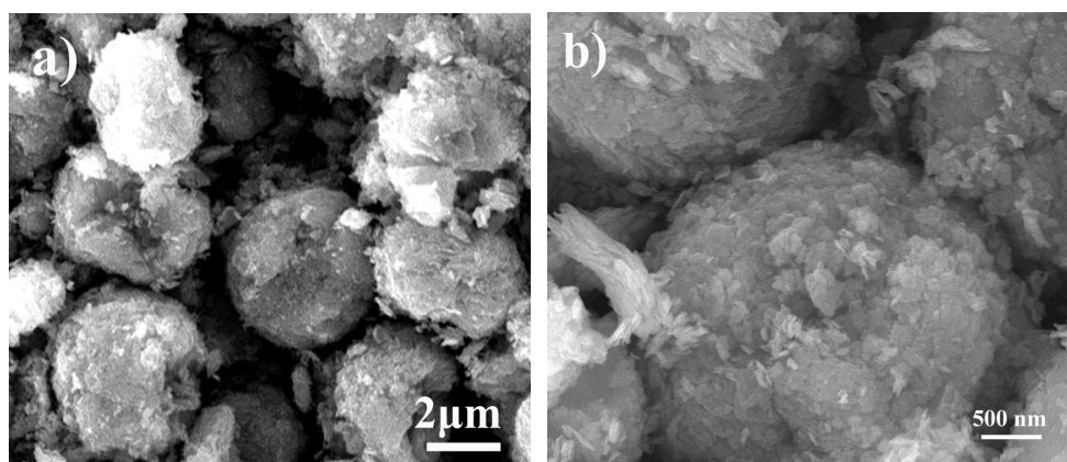
Figure S1. SEM images of the NiO product obtained by annealing of Ni(OH) 2 .
