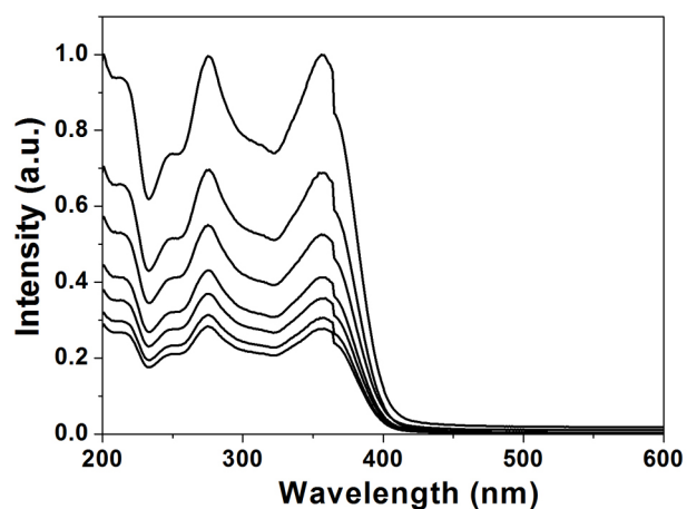
Fig. S1 Absorption spectra of TC with different irradiation time in the presence of Fe-Ti-Oxide-M (10%).
