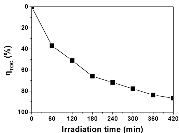
Fig. S2 TOC removal percentage in the photodegradation of TC by Fe-Ti-Oxide-M (10%).
