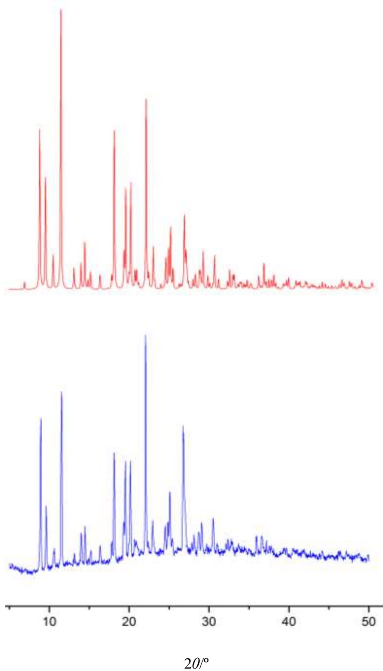
Figure S3: Simulated (Red) and powder X-ray diffraction patterns (Blue) of 3
