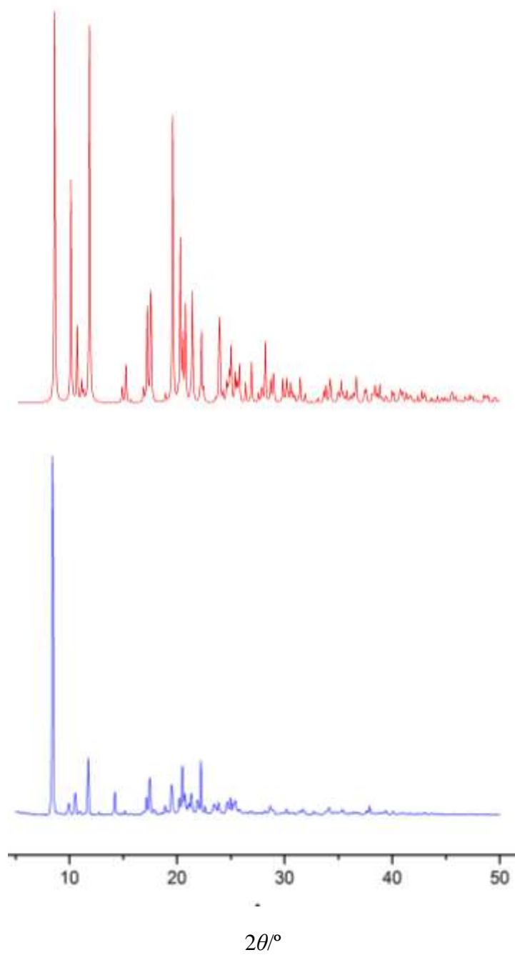
Figure S2: Simulated (Red) and powder X-ray diffraction patterns (Blue) of 2
