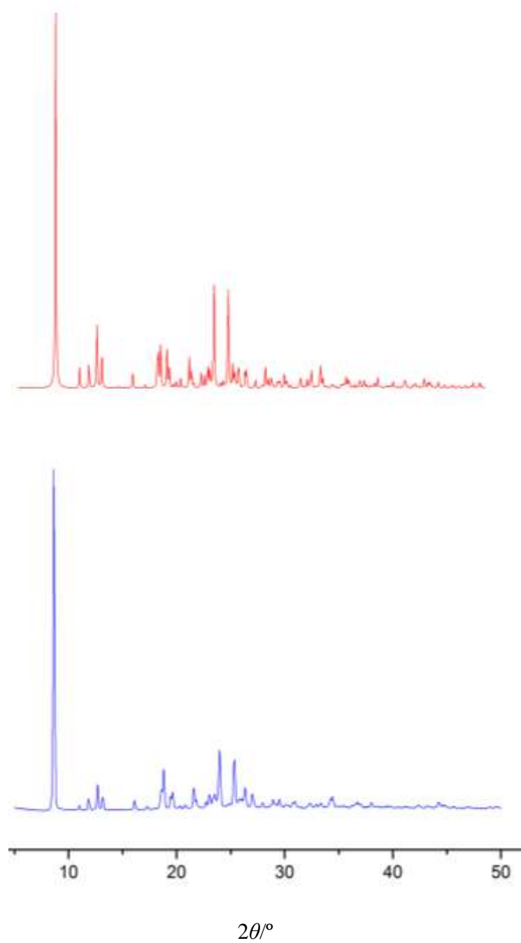
Figure S1: Simulated (Red) and powder X-ray diffraction patterns (Blue) of 1
