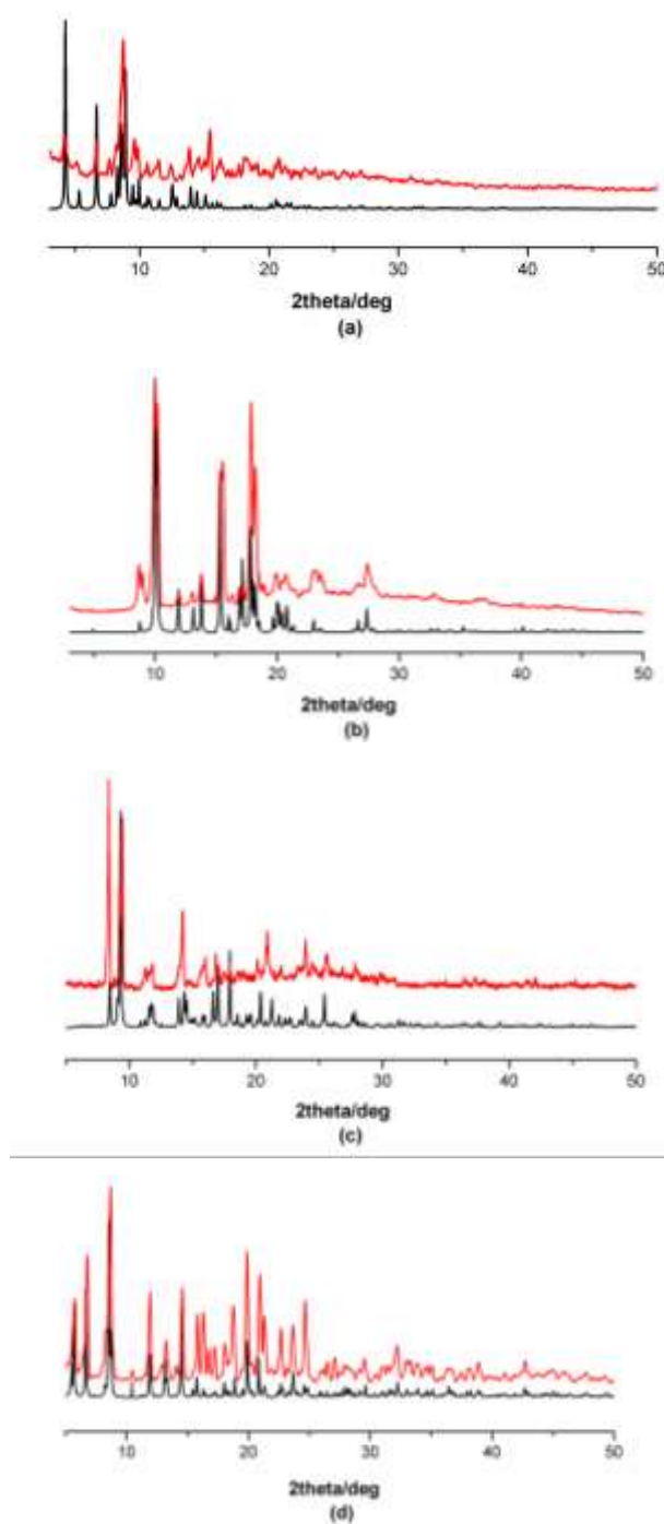
Figure S1 The X-ray powder diffraction patterns for the simulated (black), as-synthesized samples (red). (a for 1 , b for 2 , c for 3 , d for 4 )
