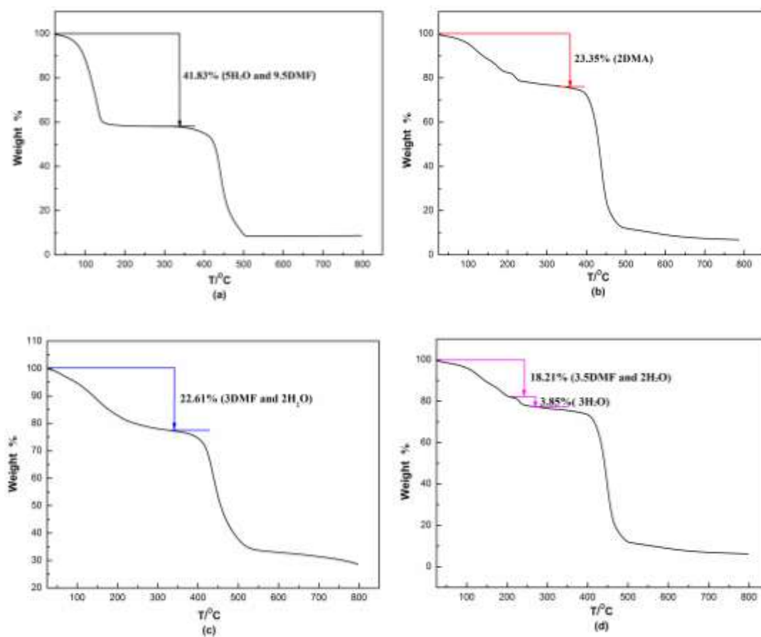
Figure S2 TGA plots of 1-4 . (a for 1 , b for 2 , c for 3 , d for 4 )
