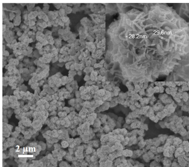
Fig. SI-1. SEM images of the Cu 3 BiS 3 powders by solvothermal route at 180 °C for 3 h and 6h.
