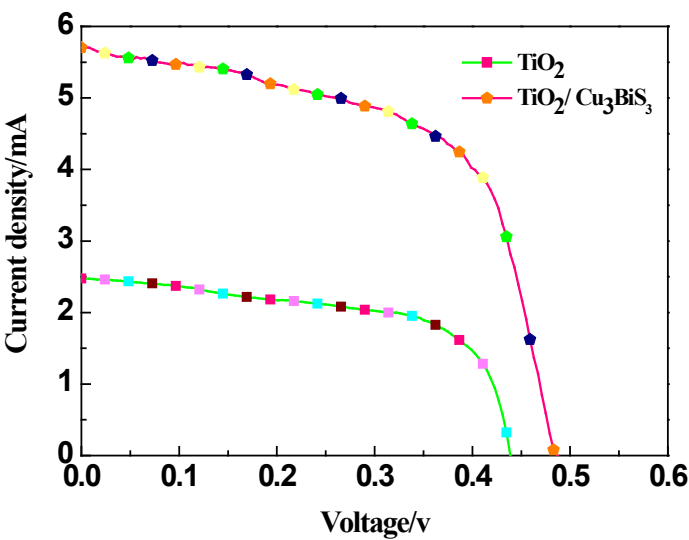
Fig. SI-2. photocurrent–voltage curves of the Cu 3 BiS 3 /TiO 2 composite film and TiO 2 film.
