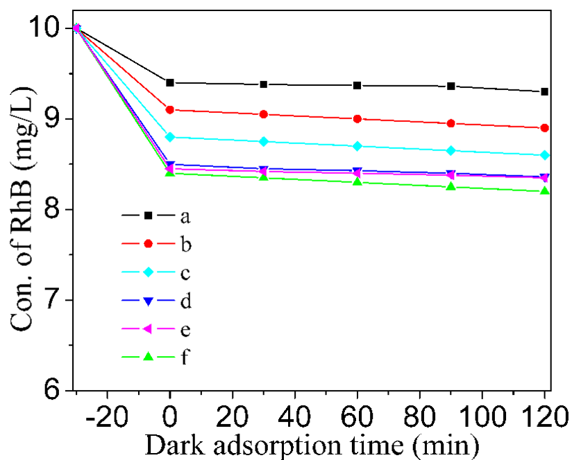
Fig. S1 Dark adsorption curves of the different samples: \text{Bi}_2\text{MoO}_6 (a), hierarchical RGO/ \text{Bi}_2\text{MoO}_6 composites with different GO contents: 2 wt% (b), 3 wt% (c), 4 wt% (d), the mixture of 4 wt% RGO and \text{Bi}_2\text{MoO}_6 generated by mechanically mixing (e) and 5 wt% (f),
