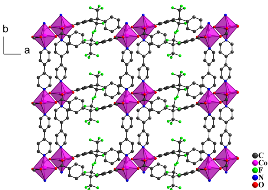
Fig. S1 A view of the double square layer structure in compound 2a .
