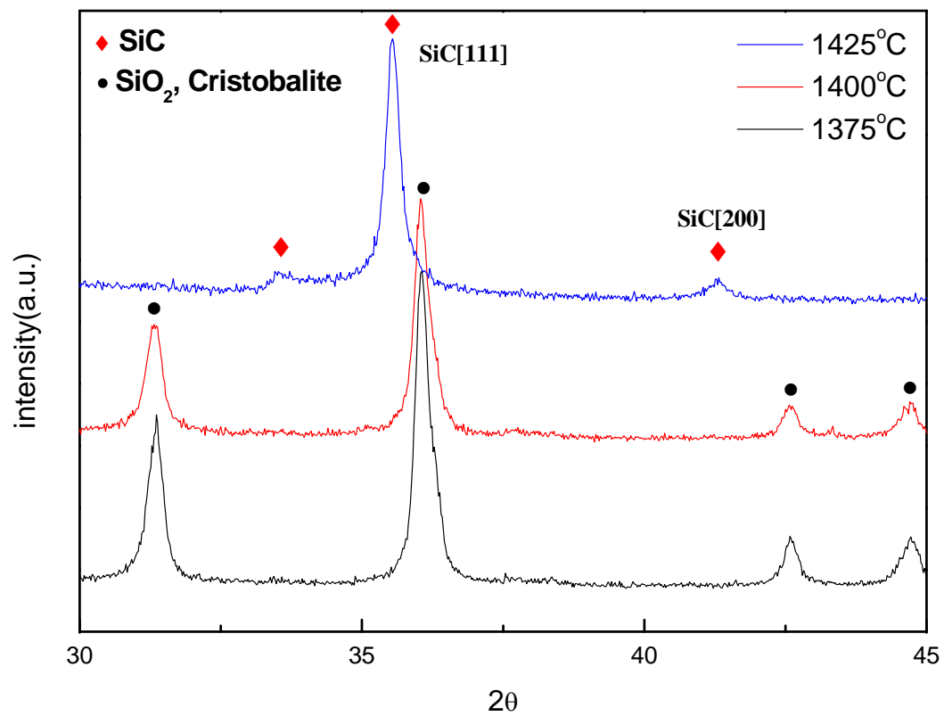
Supplementary Figure 1. X-ray diffraction patterns for the samples produced at 1370°C, 1400°C and 1425°C , respectively.
