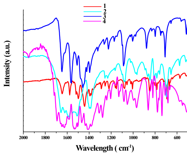
Fig. S3 The IR spectra of the title compounds.
