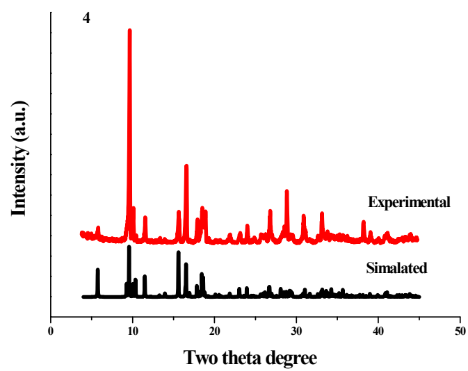
Fig. S4 The simulated (black) and experimental (red) powder XRD patterns for the title compounds.
