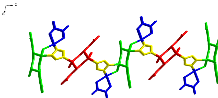
Fig S1 The projection plot of compound 4 in (010) direction.
