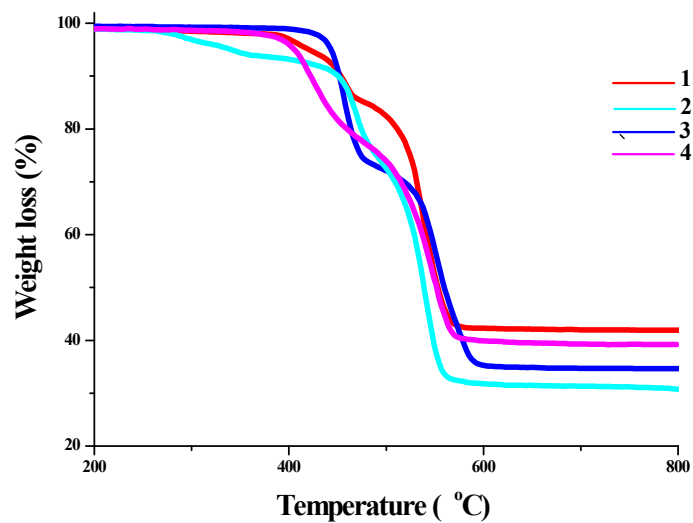
Fig. S2 The TG curve of compounds 1-4.
