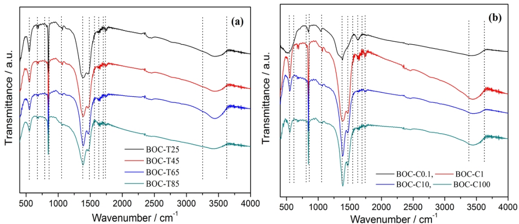
Fig. S1 FT-IR spectra of the samples obtained at different temperature (a) and different CO 2 concentration (b).
