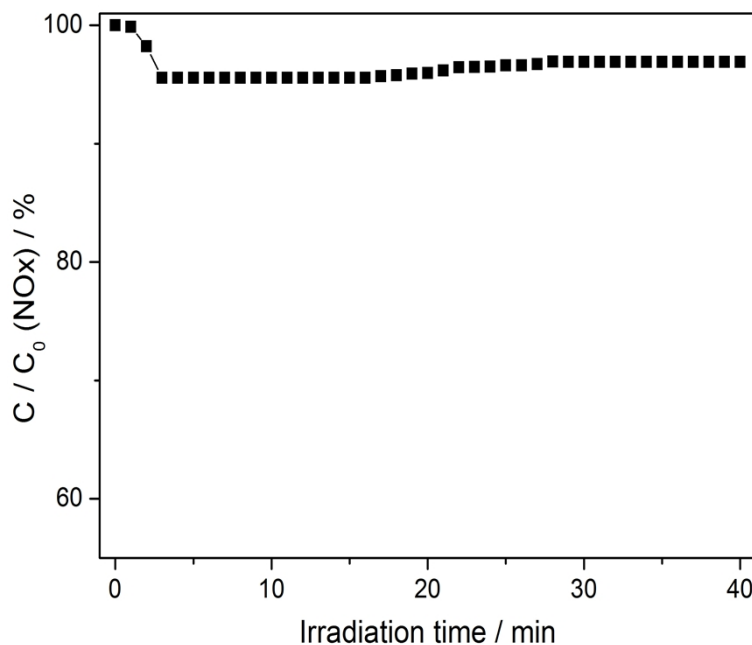
Fig. S2 Photocatalytic removal of NO x of the (BiO) 2 CO 3 sample under visible light irradiation.
