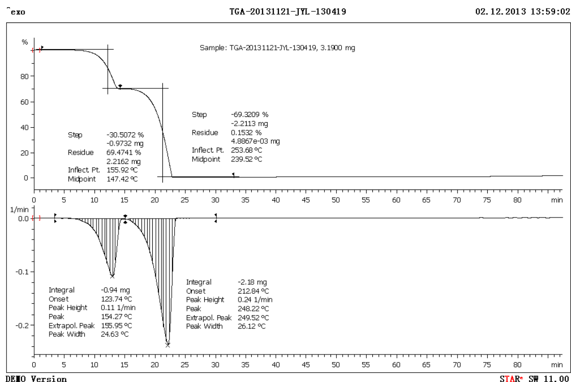
The TGA and DSC curves of 2
