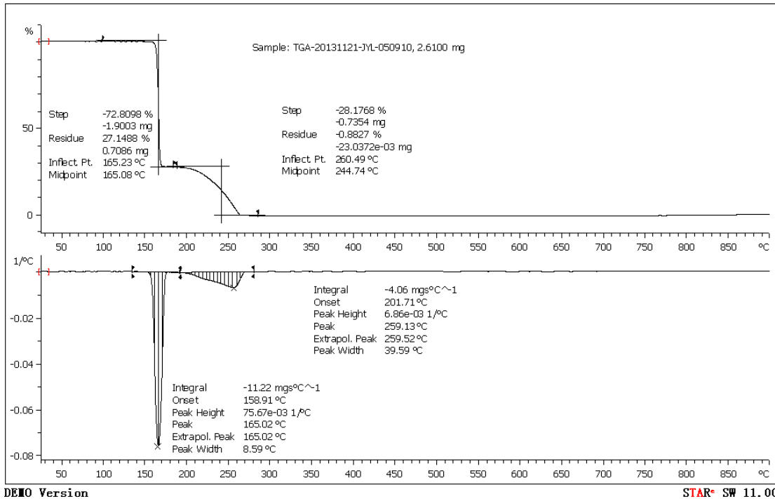
The TGA and DSC curves of 6
