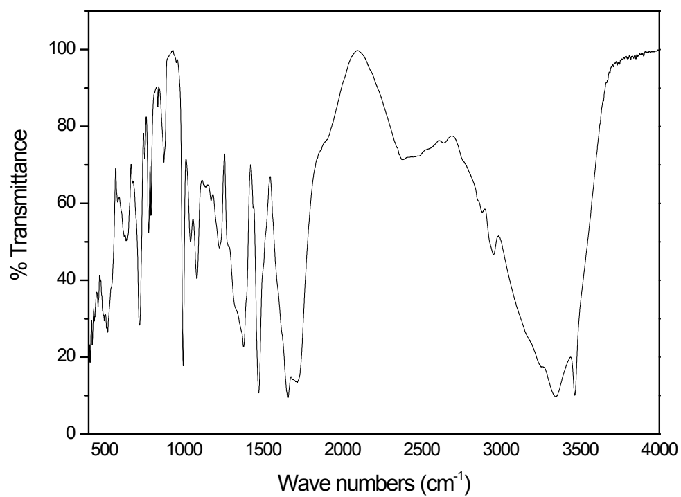
The IR curve of 8
