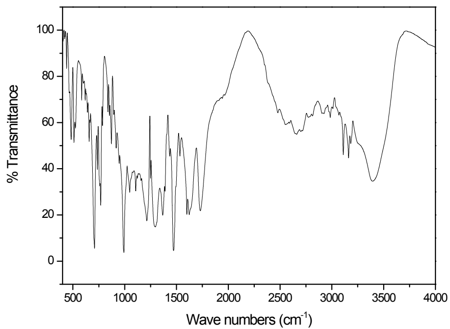
The IR curve of 6
