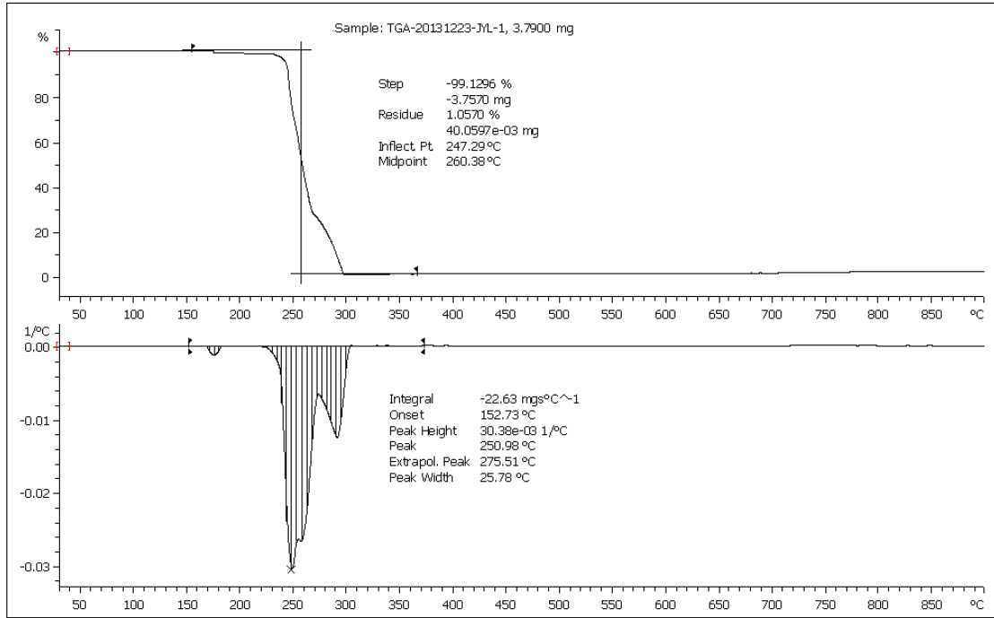
The TGA and DSC curves of 7
