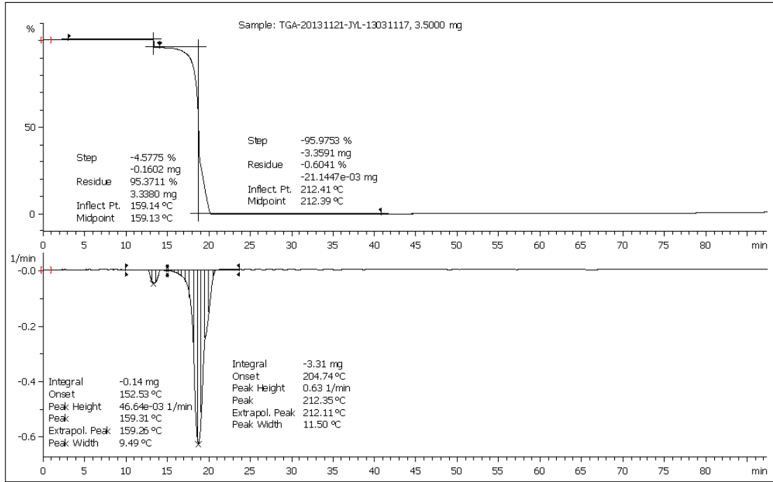
The TGA and DSC curves of 5
