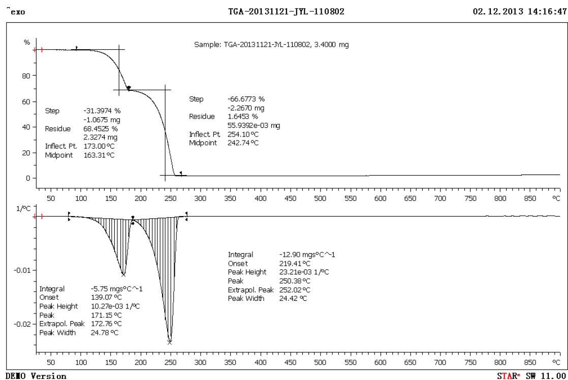
The TGA and DSC curves of 1
