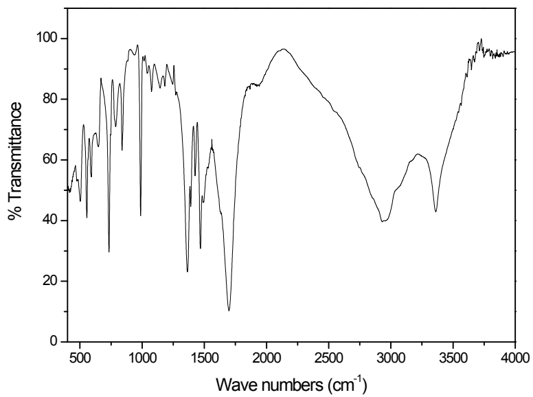
The IR curve of 3
