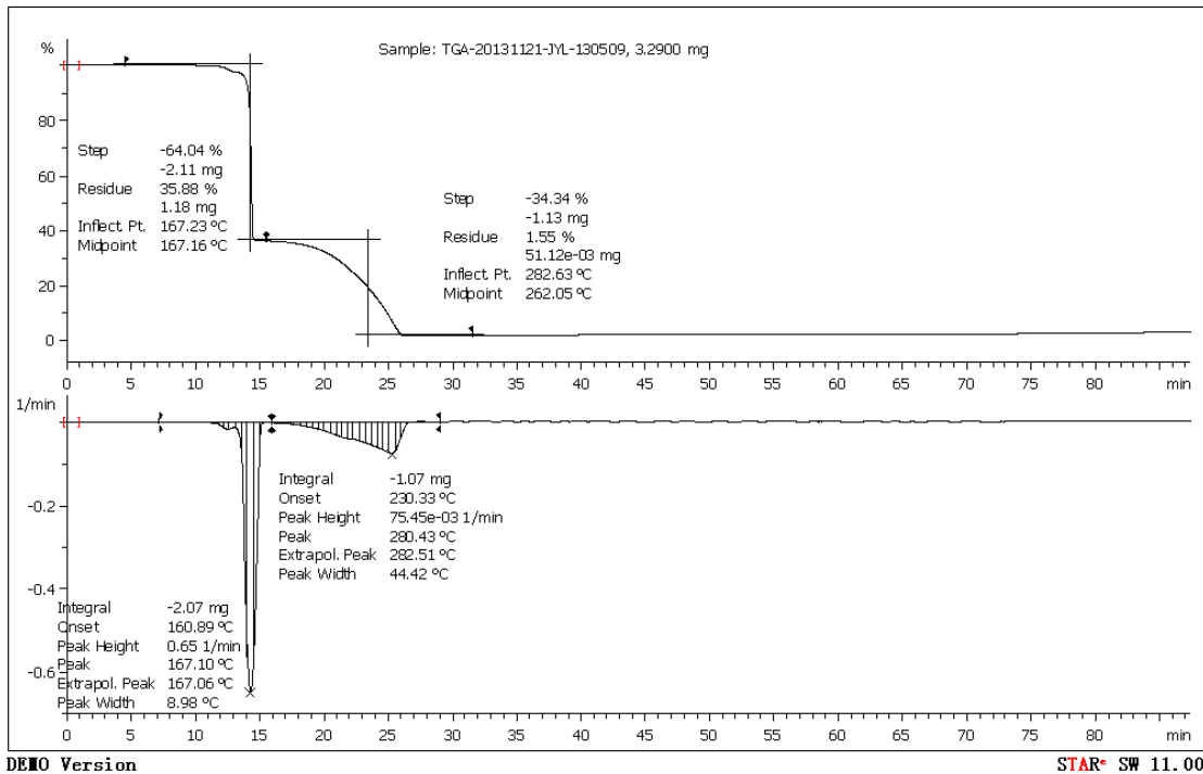
The TGA and DSC curves of 8
