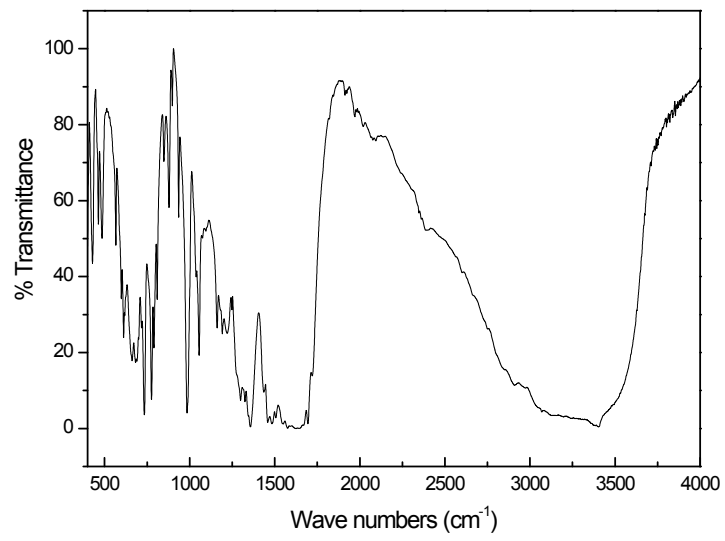
The IR curve of 4
