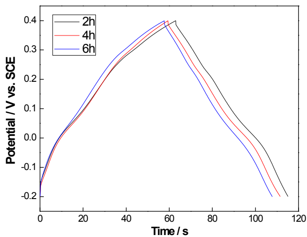
Fig. S2 GCD curves of S-PVP under reaction time of 2 h, 4 h, and 6 h
