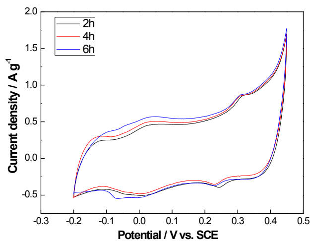
Fig. S1 CV curves of S-PVP under reaction time of 2 h, 4 h, and 6 h
