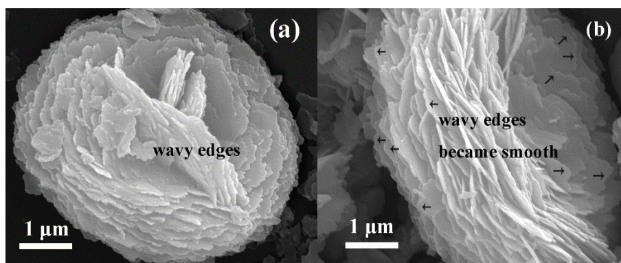
Fig. S2 WF1 sample, (a) reaction time is 3h. (b) reaction time is 5h. Wavy edges of petals begun become smooth prolong the reaction time.
