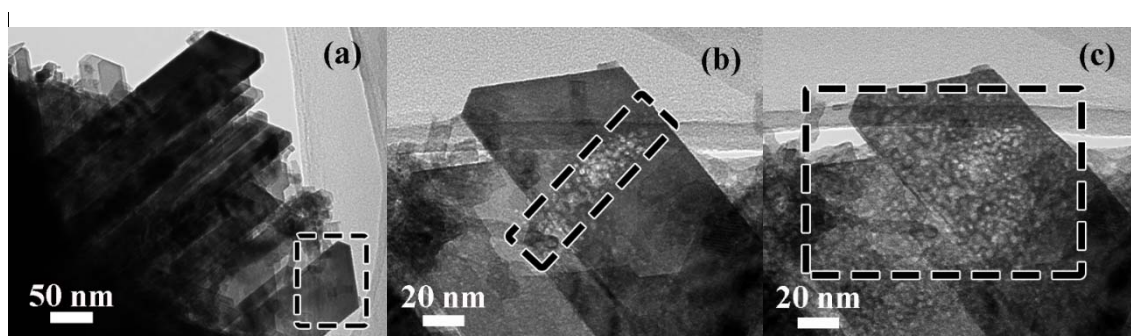
Fig. S1 surface of the sample aperture appeared with the extension of the electron beam irradiation time, due to loss of crystal water.
