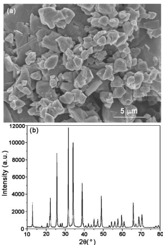
Fig. S1. FESEM image (a) and XRD pattern (b) of the Zn 2 SiO 4 bulk particles.
