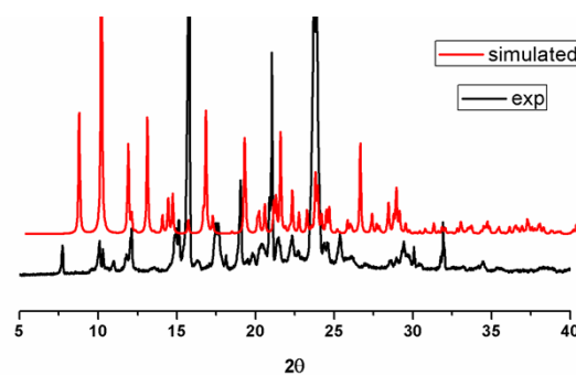
Figure S3. The experimental XRD pattern (black) and simulated XRD pattern from single crystal data (red) of 6 .
