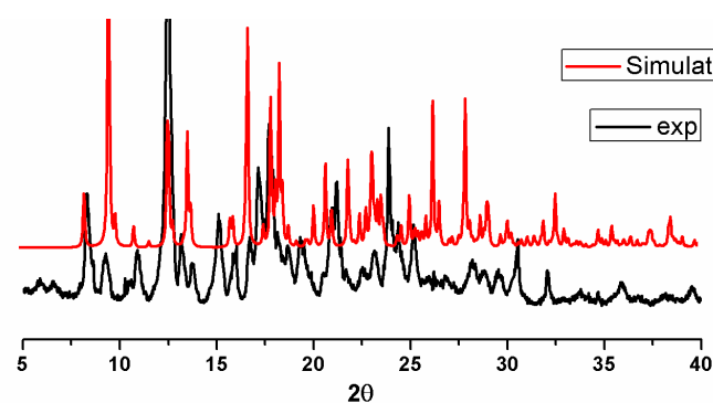
Figure S2. The experimental XRD pattern (black) and simulated XRD pattern from single crystal data (red) of 5 .
