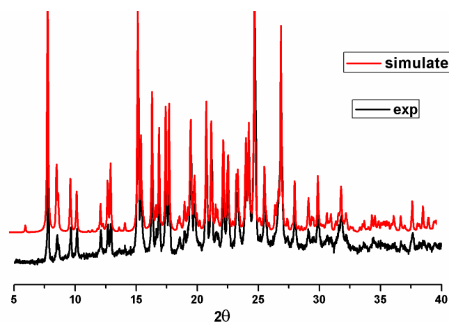
Figure S1. The experimental XRD pattern (black) and simulated XRD pattern from single crystal data (red) of 4 .
