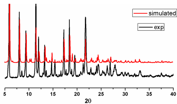
Figure S4. The experimental XRD pattern (black) and simulated XRD pattern from single crystal data (red) of 7 .
