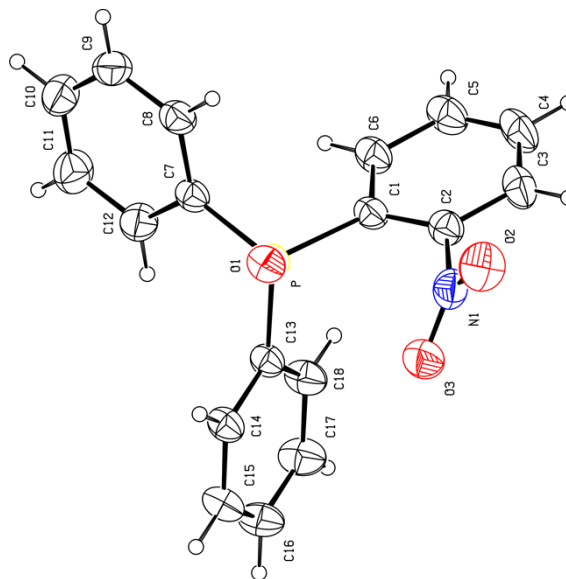
Figure 2. ORTEP representation of Form II
