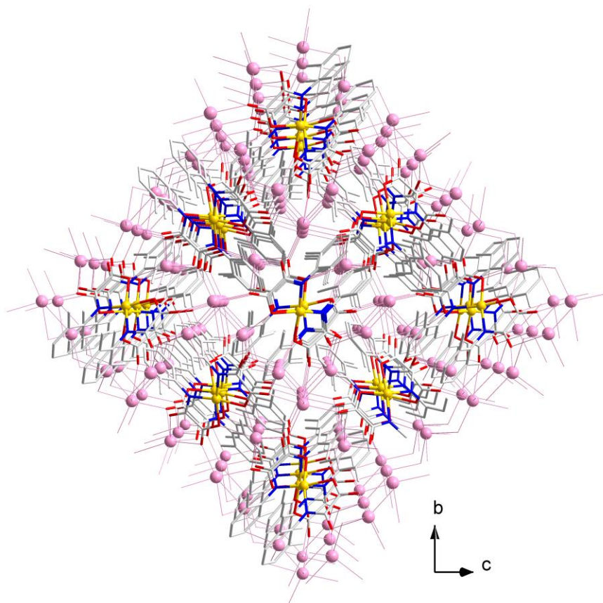
Figure S1. Perspective view of the crystal packing of 1b along the crystallographic a axis.
