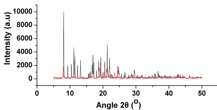
Figure S6. XRPD patterns of the complex 7 crystals (red), compared with the simulated XRPD pattern of complex 7 (back).
