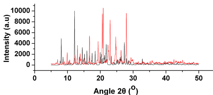
Figure S2. XRPD patterns of the complex 2 crystals (red), compared with the simulated XRPD pattern of complex 2 (black).
