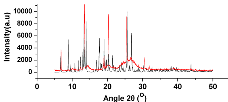
Figure S1. XRPD patterns of the complex 1 crystals (red), compared with the simulated XRPD pattern of complex 1 (black).
