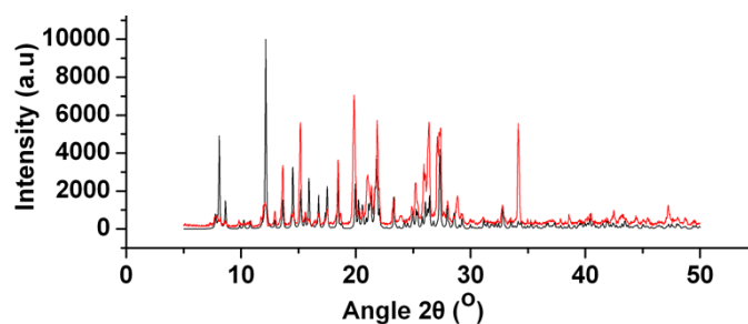
Figure S3. XRPD patterns of the complex 3 crystals (red), compared with the simulated XRPD pattern of complex 3 (black).
