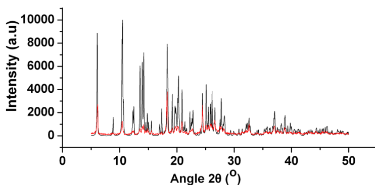
Figure S5. XRPD patterns of the complex 6 crystals (red), compared with the simulated XRPD pattern of complex 6 (back).
