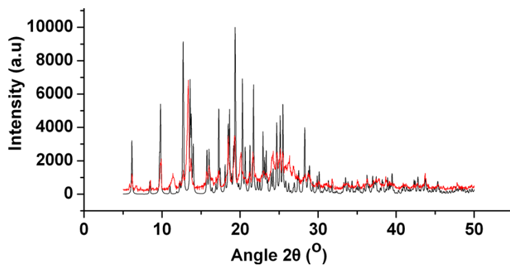
Figure S4. XRPD patterns of the complex 4 crystals (red), compared with the simulated XRPD pattern of complex 4 (back).
