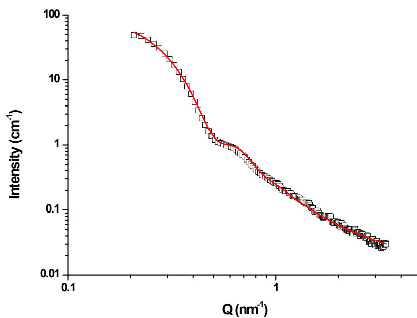
Figure S1. SAXS profile of the U(IV)-based sample heated at 90°C for 120 min (squares). The red line represents the calculation of the form factor of spheres with a diameter of 16.4 nm (FWHM = 5 nm).
