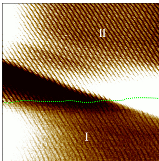
Fig. S1 Large-scale STM image of C2 self-assembly at 1-phenyloctane/ HOPG interface showing the coexistence of two types of structures (Type I and Type II). Scan area: 200 nm × 200 nm; Tunneling conditions: V_{\text{bias}} = 764 mV, I_t = 482 pA.
