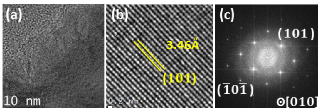
Figure S1. TEM image of pristine \text{TiO}_2 nanofibre catalysts (a) , and its high-magnification of the lattice (b) with the corresponding fast Fourier transformed pattern of this specimen (c) .
