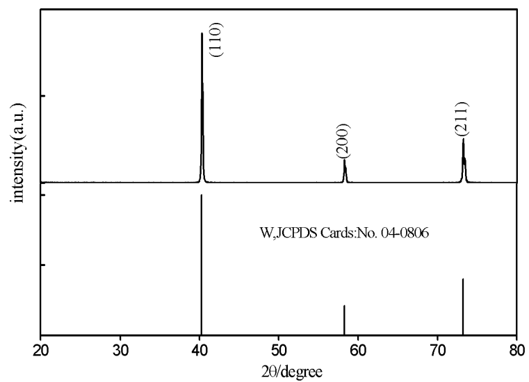
Fig. S1 XRD spectrum of the tungsten powder
