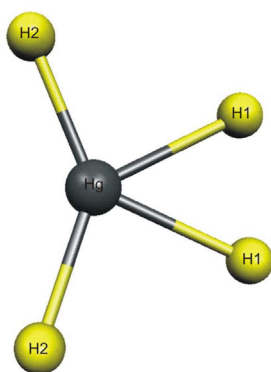
Fig. S1: The structure of transition state for \text{HgH}_4 dissociation.
