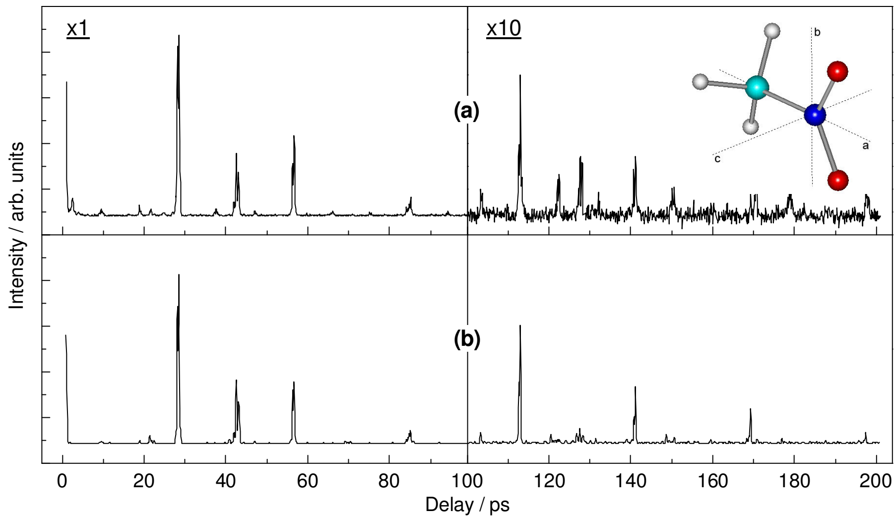
Picture. Experimental (a) and simulated (b) fs DFWM spectra of nitromethane
