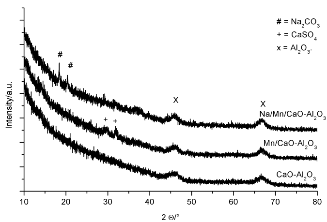
Fig. S2 XRD patterns for samples not treated with H 2 O
