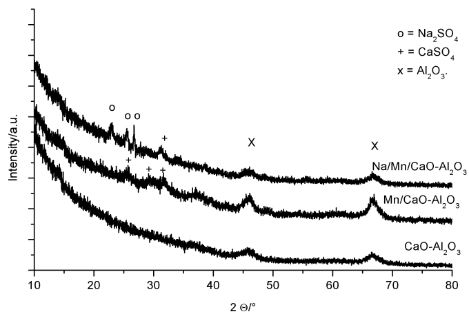
Fig. S1 XRD patterns for samples treated with H 2 O.
