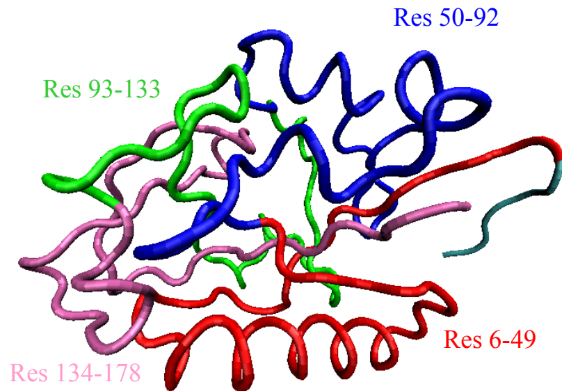
Supplementary figure 1. Human endostatin structure. Fragments 6-49 (red), 50-92 (blue), 93-133 (green) and 134-178 (mauve) are shown.
