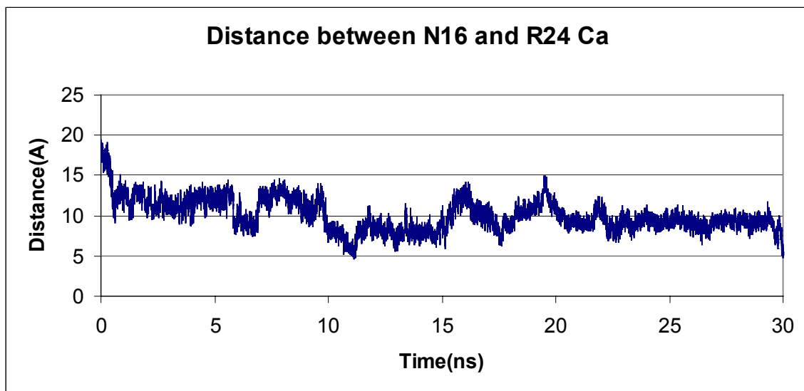
Supplementary figure 3. Distance between the Ca atoms of N 16 and R 24 .
