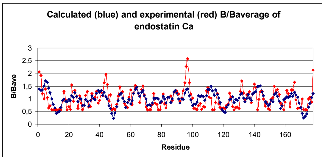
Supplementary figure 2. Calculated (blue) and experimental (red) values of B/B_{\text{average}} for C_{\alpha} carbons of full-length hE.
