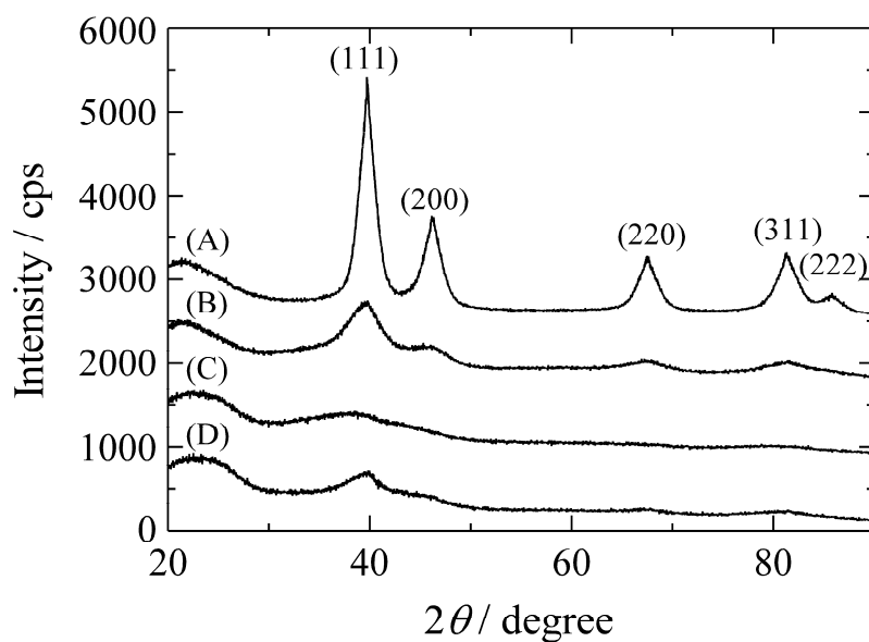
Figure XRD patterns for Pt(4.8 nm)/CB (line A), Pt(2.6 nm)/CB (line B), (1.6 nm)/CB (line C), Pt(2.6 nm)/CB with the same Pt loading as 1.6 nm size catalyst (line D).
