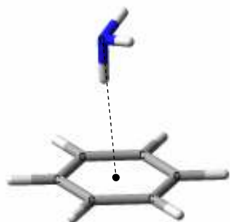
Benzene·NH 3 ( C_s )
