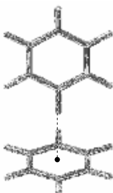
Benzene dimer ( C_{2v} )
