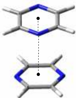
Pyrazine dimer ( C_s )
