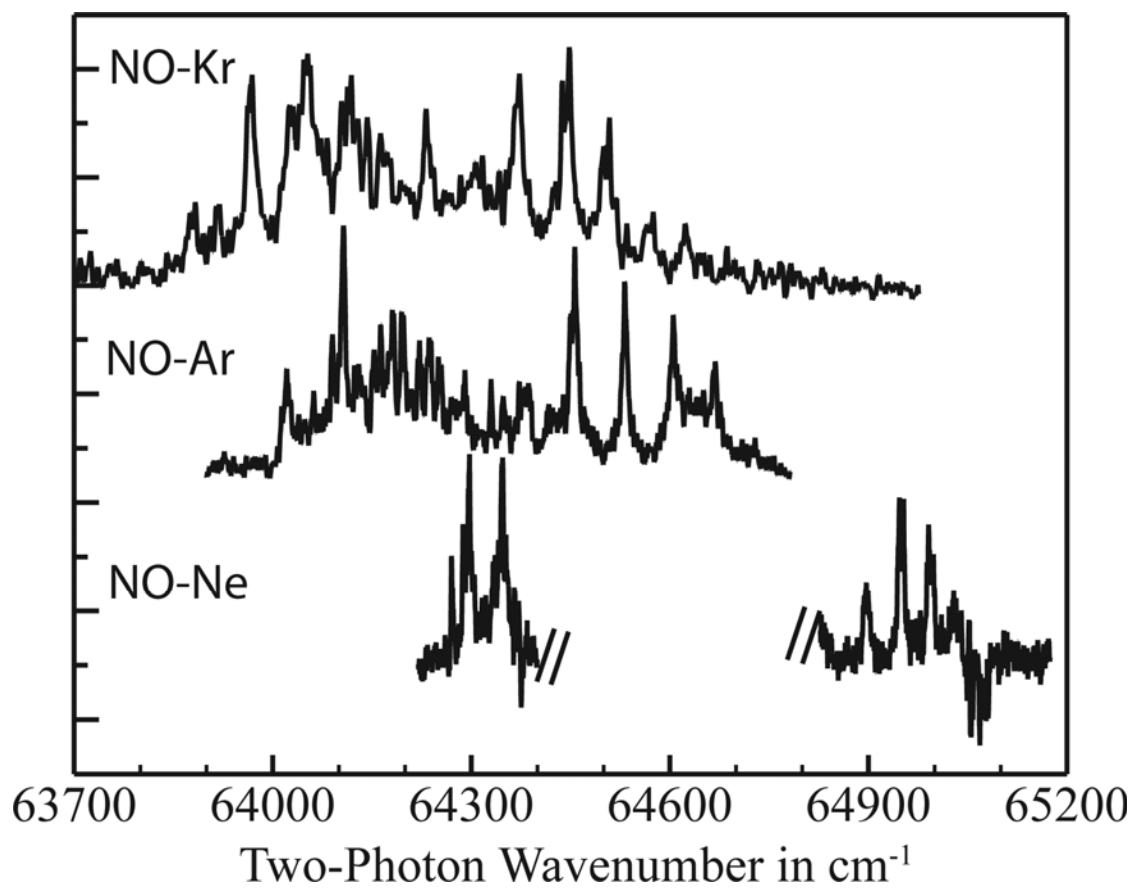
Fig. S1: Spectra of the \tilde{H}' , \tilde{F} \leftarrow \tilde{X} transitions in the NO-Rg complexes.
